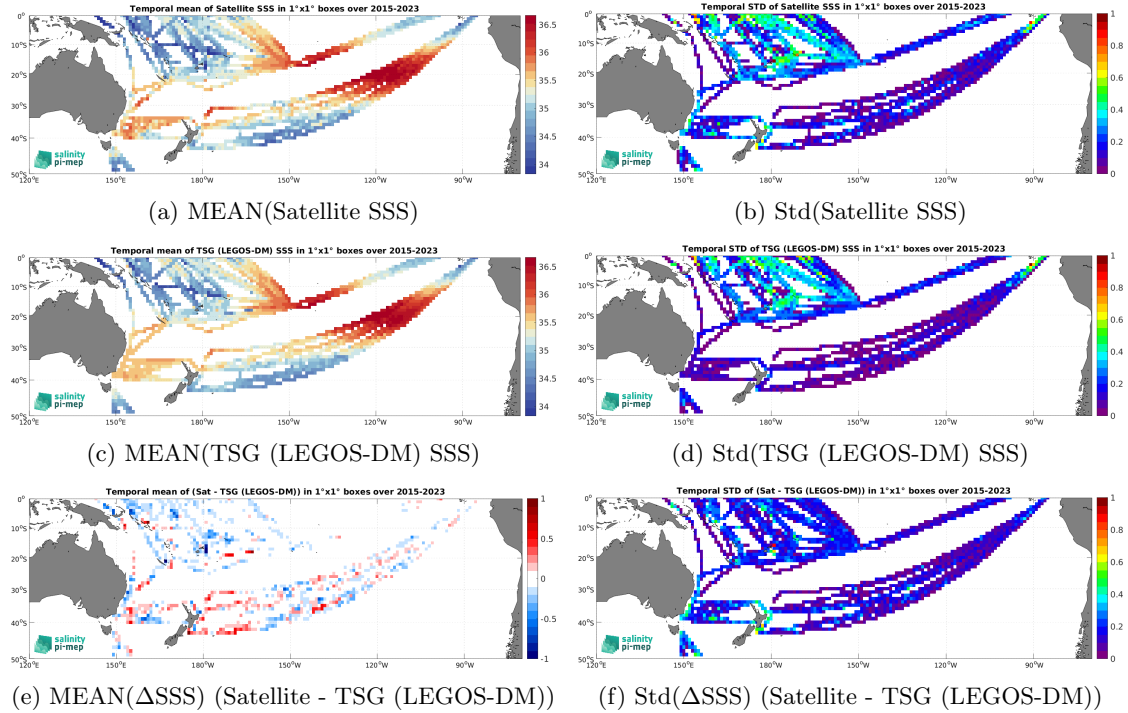
Figure 7: Temporal mean (left) and Std (right) of SSS from SMAP SSS L3 v5.3 - 8-Day running (RSS) (top), TSG (LEGOS-DM) (middle), and of \Delta\text{SSS} (Satellite - TSG (LEGOS-DM)). Only match-up pairs are used to generate these maps.
