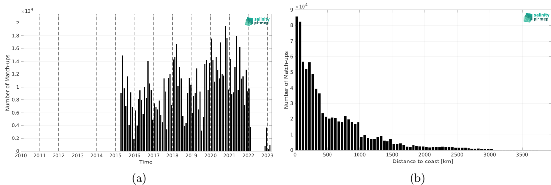
Figure 2: Number of match-ups between TSG (LEGOS-DM) and SMAP SSS L3 v5.3 - 8-Day running (RSS) SSS as a function of time (a) and as function of the distance to coast (b) over the South Pacific Ocean Pi-MEP region and for the full satellite product period.
