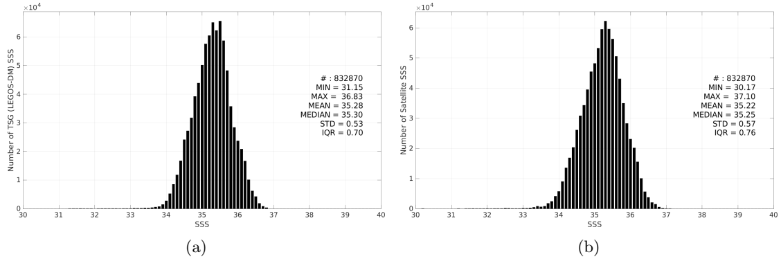
Figure 3: Histograms of SSS from TSG (LEGOS-DM) (a) and SMAP SSS L3 v5.3 - 8-Day running (RSS) (b) considering all match-up pairs per bins of 0.1 over the South Pacific Ocean Pi-MEP region and for the full satellite product period.
