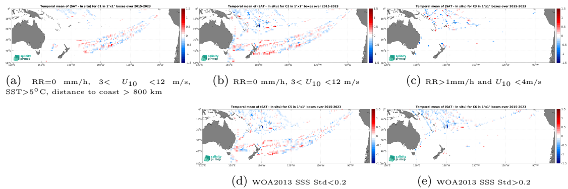
Figure 14: Temporal mean gridded over spatial boxes of size 1^\circ \times 1^\circ of \Delta SSS (SMAP SSS L3 v5.3 - 8-Day running (RSS) - TSG (LEGOS-DM)) for 5 different subdatasets corresponding to:RR=0 mm/h, 3 < U_{10} < 12 m/s, SST>5°C, distance to coast > 800 km (a), RR=0 mm/h, 3 < U_{10} < 12 m/s (b), RR>1mm/h and U_{10} < 4 m/s (c), WOA2013 SSS Std<0.2 (d), WOA2013 SSS Std>0.2 (e).
