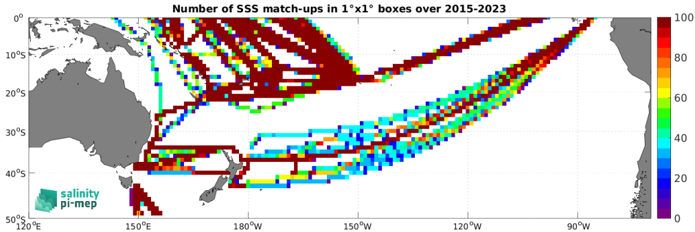
Figure 5: Number of SSS match-ups between TSG (LEGOS-DM) SSS and the SMAP SSS L3 v5.3 - 8-Day running (RSS) SSS product for the South Pacific Ocean Pi-MEP region over 1^\circ \times 1^\circ boxes and for the full satellite product period.
