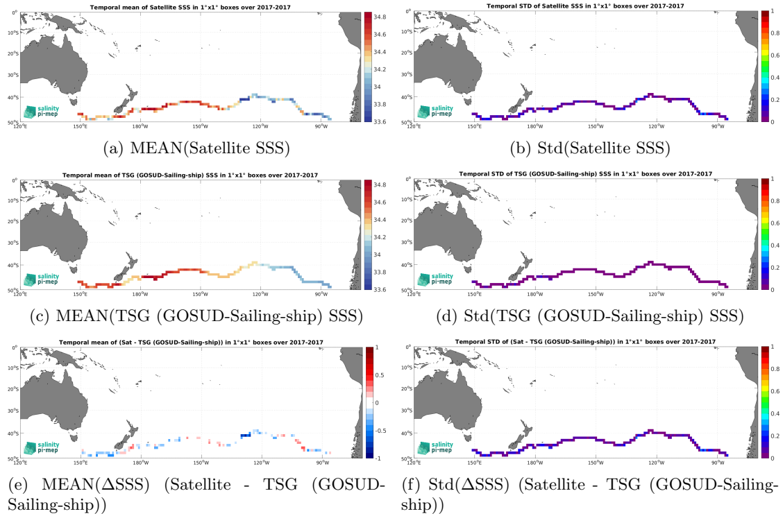
Figure 7: Temporal mean (left) and Std (right) of SSS from SMAP SSS L3 v5.3 - 8-Day running (RSS) (top), TSG (GOSUD-Sailing-ship) (middle), and of \Delta SSS (Satellite - TSG (GOSUD-Sailing-ship)). Only match-up pairs are used to generate these maps.
