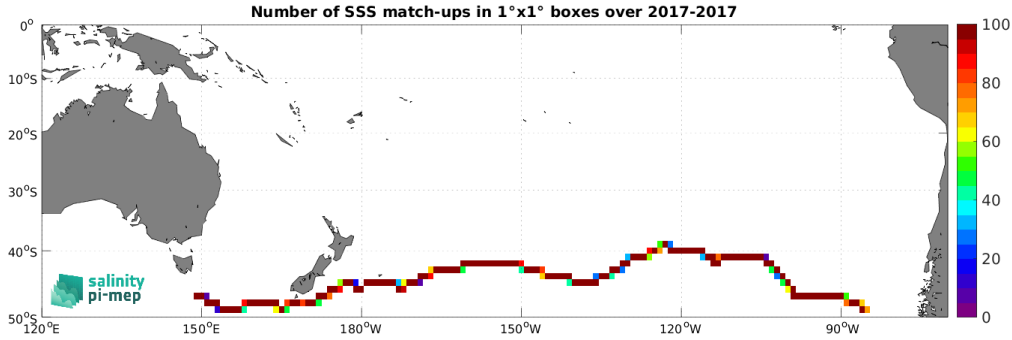
Figure 5: Number of SSS match-ups between TSG (GOSUD-Sailing-ship) SSS and the SMAP SSS L3 v5.3 - 8-Day running (RSS) SSS product for the South Pacific Ocean Pi-MEP region over 1^\circ \times 1^\circ boxes and for the full satellite product period.
