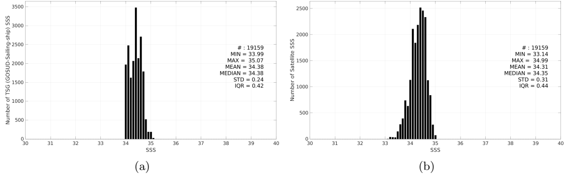
Figure 3: Histograms of SSS from TSG (GOSUD-Sailing-ship) (a) and SMAP SSS L3 v5.3 - 8-Day running (RSS) (b) considering all match-up pairs per bins of 0.1 over the South Pacific Ocean Pi-MEP region and for the full satellite product period.
