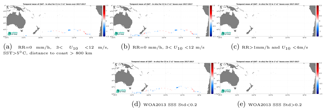
Figure 14: Temporal mean gridded over spatial boxes of size 1^\circ \times 1^\circ of \Delta SSS (SMAP SSS L3 v5.3 - 8-Day running (RSS) - TSG (GOSUD-Sailing-ship)) for 5 different subdatasets corresponding to:RR=0 mm/h, 3 < U_{10} < 12 m/s, SST >5^\circ\text{C} , distance to coast > 800 km (a), RR=0 mm/h, 3 < U_{10} < 12 m/s (b), RR >1 mm/h and U_{10} < 4 m/s (c), WOA2013 SSS Std <0.2 (d), WOA2013 SSS Std >0.2 (e).
