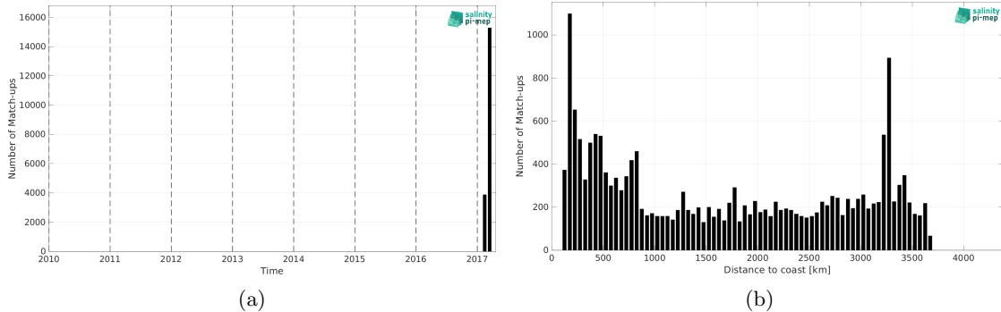
Figure 2: Number of match-ups between TSG (GOSUD-Sailing-ship) and SMAP SSS L3 v5.3 - 8-Day running (RSS) SSS as a function of time (a) and as function of the distance to coast (b) over the South Pacific Ocean Pi-MEP region and for the full satellite product period.
