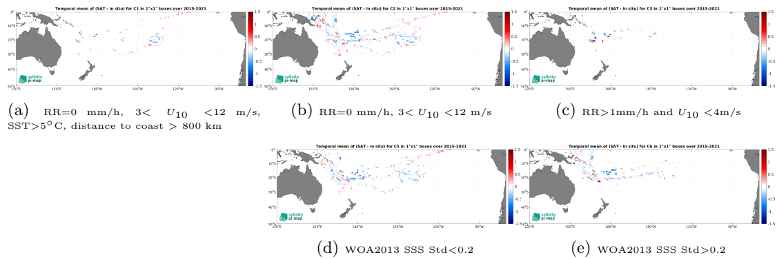
Figure 14: Temporal mean gridded over spatial boxes of size 1^\circ \times 1^\circ of \Delta\text{SSS} (SMAP SSS L3 v5.3 - 8-Day running (RSS) - TSG (GOSUD-Research-vessel)) for 5 different subdatasets corresponding to:RR=0 mm/h, 3 < U_{10} < 12 m/s, SST>5°C, distance to coast > 800 km (a), RR=0 mm/h, 3 < U_{10} < 12 m/s (b), RR>1mm/h and U_{10} < 4 m/s (c), WOA2013 SSS Std<0.2 (d), WOA2013 SSS Std>0.2 (e).
