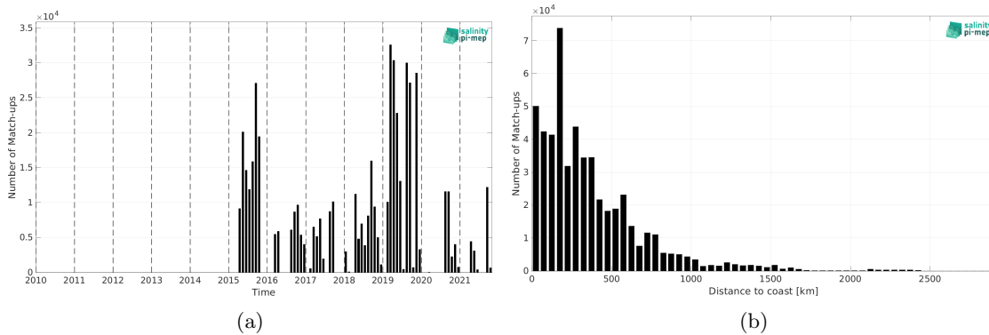
Figure 2: Number of match-ups between TSG (GOSUD-Research-vessel) and SMAP SSS L3 v5.3 - 8-Day running (RSS) SSS as a function of time (a) and as function of the distance to coast (b) over the South Pacific Ocean Pi-MEP region and for the full satellite product period.
