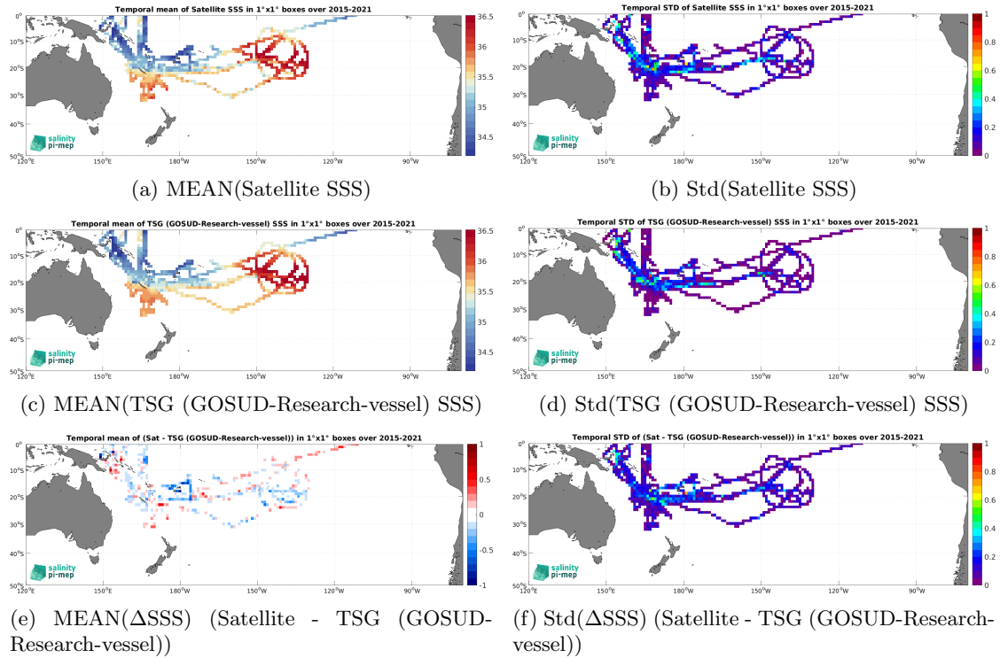
Figure 7: Temporal mean (left) and Std (right) of SSS from SMAP SSS L3 v5.3 - 8-Day running (RSS) (top), TSG (GOSUD-Research-vessel) (middle), and of \Delta SSS (Satellite - TSG (GOSUD-Research-vessel)). Only match-up pairs are used to generate these maps.
