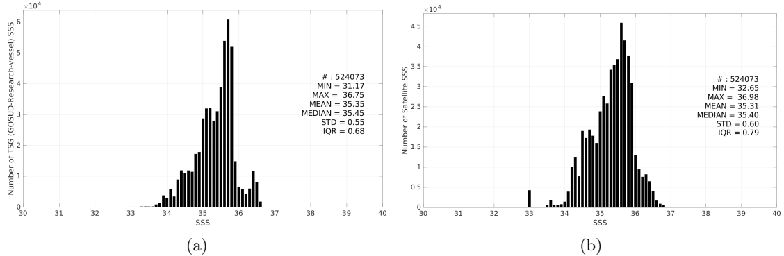
Figure 3: Histograms of SSS from TSG (GOSUD-Research-vessel) (a) and SMAP SSS L3 v5.3 - 8-Day running (RSS) (b) considering all match-up pairs per bins of 0.1 over the South Pacific Ocean Pi-MEP region and for the full satellite product period.
