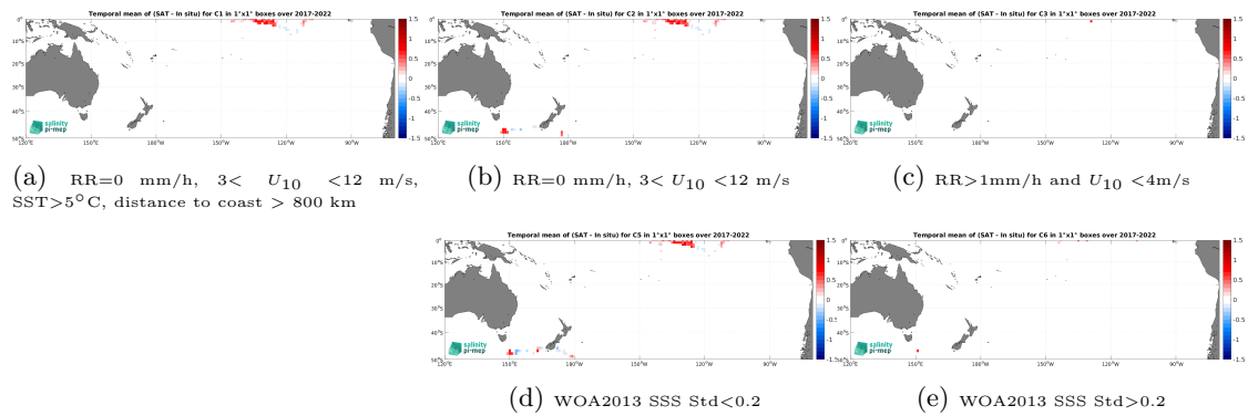
Figure 14: Temporal mean gridded over spatial boxes of size 1^\circ \times 1^\circ of \Delta SSS (SMAP SSS L3 v5.3 - 8-Day running (RSS) - Saildrone) for 5 different subdatasets corresponding to:RR=0 mm/h, 3 < U_{10} < 12 m/s, SST >5^\circ\text{C} , distance to coast > 800 km (a), RR=0 mm/h, 3 < U_{10} < 12 m/s (b), RR >1 mm/h and U_{10} < 4 m/s (c), WOA2013 SSS Std <0.2 (d), WOA2013 SSS Std >0.2 (e).
