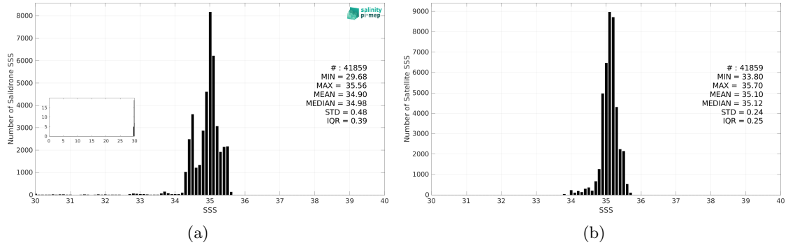
Figure 3: Histograms of SSS from Sailability (a) and SMAP SSS L3 v5.3 - 8-Day running (RSS) (b) considering all match-up pairs per bins of 0.1 over the South Pacific Ocean Pi-MEP region and for the full satellite product period.
