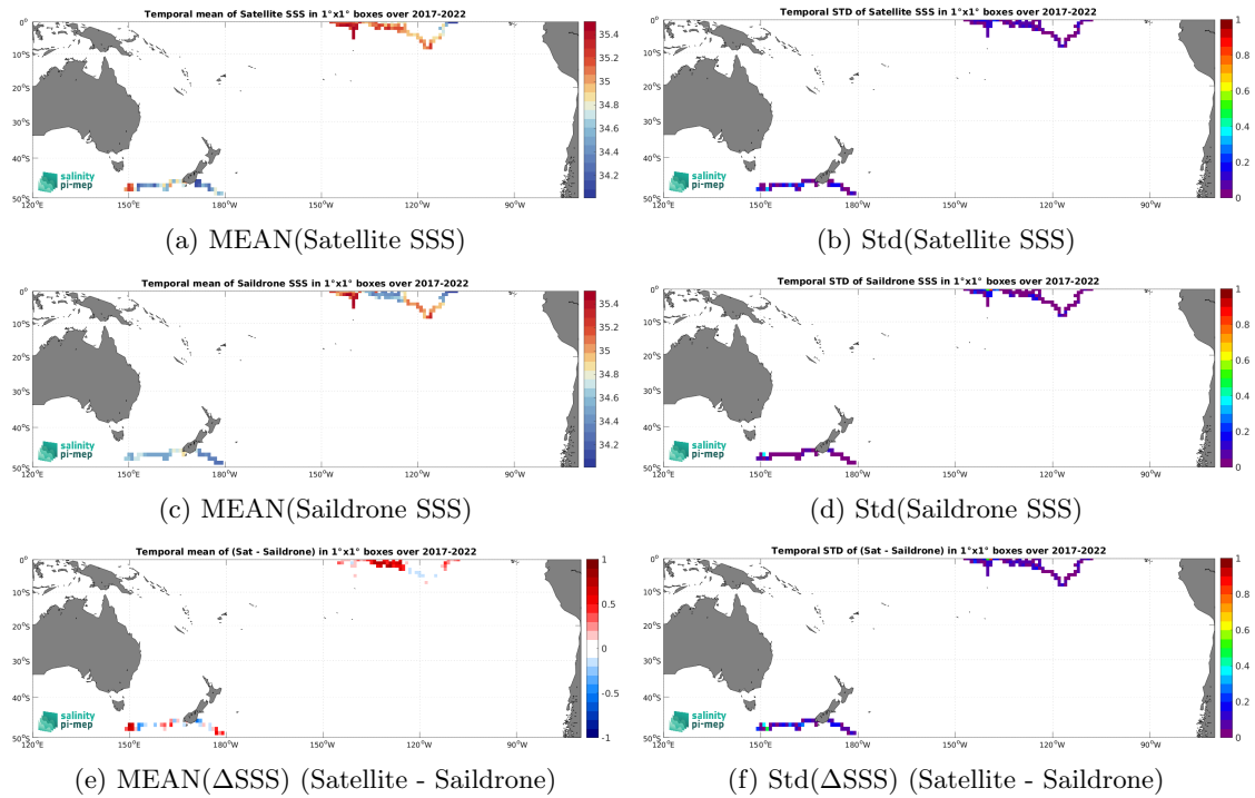
Figure 7: Temporal mean (left) and Std (right) of SSS from SMAP SSS L3 v5.3 - 8-Day running (RSS) (top), Saildrone (middle), and of \Delta SSS (Satellite - Saildrone). Only match-up pairs are used to generate these maps.
