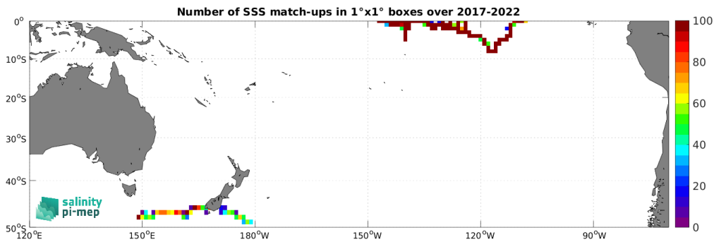
Figure 5: Number of SSS match-ups between Saildrone SSS and the SMAP SSS L3 v5.3 - 8-Day running (RSS) SSS product for the South Pacific Ocean Pi-MEP region over 1^\circ \times 1^\circ boxes and for the full satellite product period.
