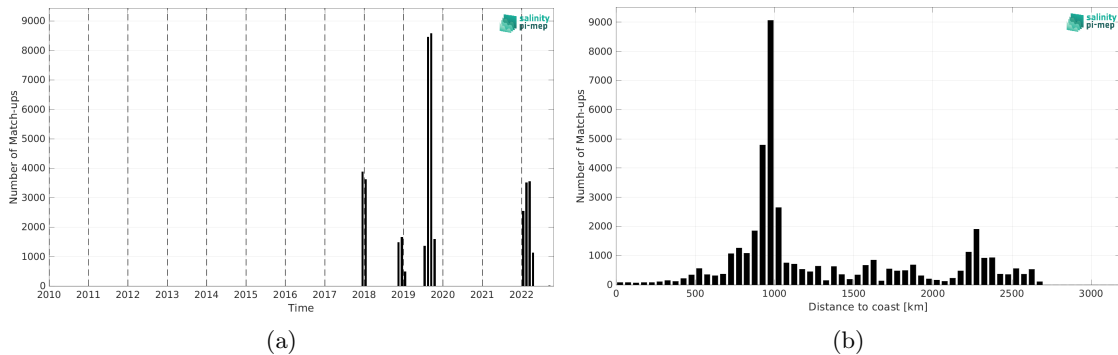
Figure 2: Number of match-ups between Saildrone and SMAP SSS L3 v5.3 - 8-Day running (RSS) SSS as a function of time (a) and as function of the distance to coast (b) over the South Pacific Ocean Pi-MEP region and for the full satellite product period.
