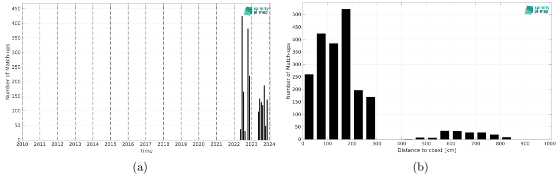
Figure 2: Number of match-ups between Marine mammals and SMAP SSS L3 v5.3 - 8-Day running (RSS) SSS as a function of time (a) and as function of the distance to coast (b) over the South Pacific Ocean Pi-MEP region and for the full satellite product period.
