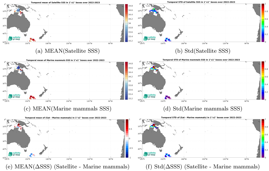
Figure 7: Temporal mean (left) and Std (right) of SSS from SMAP SSS L3 v5.3 - 8-Day running (RSS) (top), Marine mammals (middle), and of \Delta SSS (Satellite - Marine mammals). Only match-up pairs are used to generate these maps.
