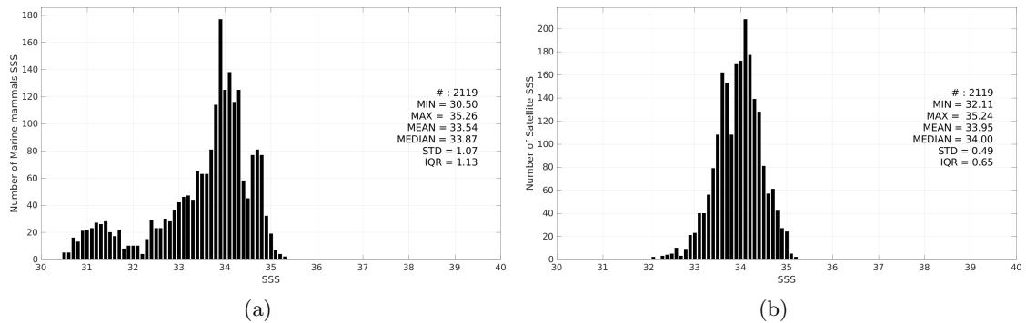
Figure 3: Histograms of SSS from Marine mammals (a) and SMAP SSS L3 v5.3 - 8-Day running (RSS) (b) considering all match-up pairs per bins of 0.1 over the South Pacific Ocean Pi-MEP region and for the full satellite product period.
