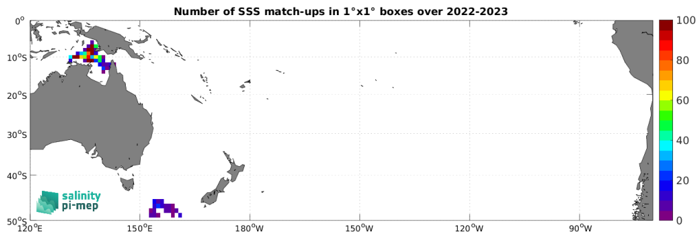
Figure 5: Number of SSS match-ups between Marine mammals SSS and the SMAP SSS L3 v5.3 - 8-Day running (RSS) SSS product for the South Pacific Ocean Pi-MEP region over 1^\circ \times 1^\circ boxes and for the full satellite product period.
