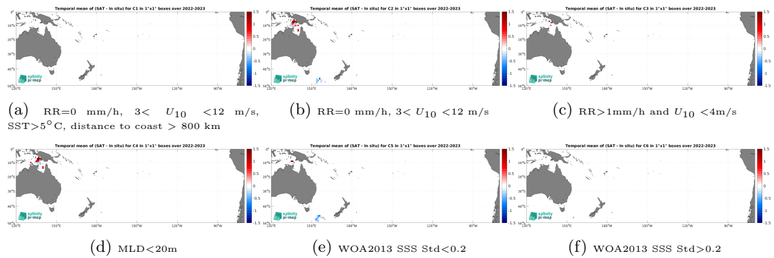
Figure 14: Temporal mean gridded over spatial boxes of size 1^\circ \times 1^\circ of \Delta SSS (SMAP SSS L3 v5.3 - 8-Day running (RSS) - Marine mammals) for 6 different subdatasets corresponding to:RR=0 mm/h, 3 < U_{10} < 12 m/s, SST >5^\circ C, distance to coast > 800 km (a), RR=0 mm/h, 3 < U_{10} < 12 m/s (b), RR >1 mm/h and U_{10} < 4 m/s (c),MLD <20 m (d),WOA2013 SSS Std <0.2 (e),WOA2013 SSS Std >0.2 (f).
