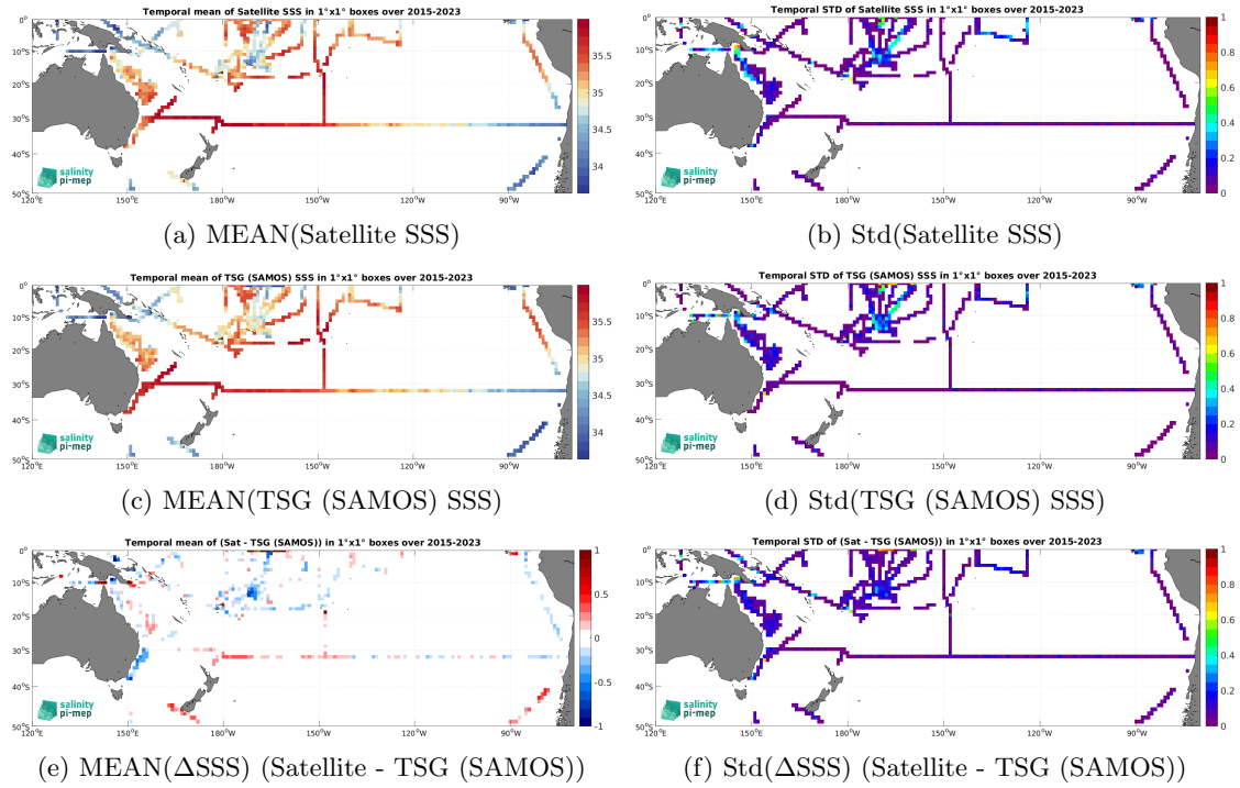
Figure 7: Temporal mean (left) and Std (right) of SSS from SMAP SSS L3 v5.3 - Monthly (RSS) (top), TSG (SAMOS) (middle), and of \Delta SSS (Satellite - TSG (SAMOS)). Only match-up pairs are used to generate these maps.
