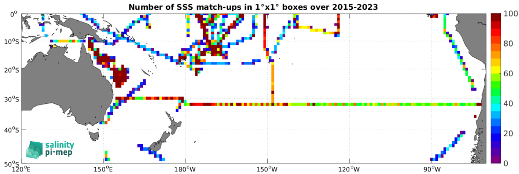
Figure 5: Number of SSS match-ups between TSG (SAMOS) SSS and the SMAP SSS L3 v5.3 - Monthly (RSS) SSS product for the South Pacific Ocean Pi-MEP region over 1^\circ \times 1^\circ boxes and for the full satellite product period.
