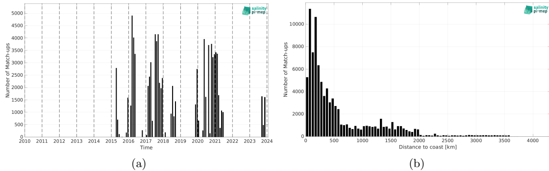
Figure 2: Number of match-ups between TSG (SAMOS) and SMAP SSS L3 v5.3 - Monthly (RSS) SSS as a function of time (a) and as function of the distance to coast (b) over the South Pacific Ocean Pi-MEP region and for the full satellite product period.
