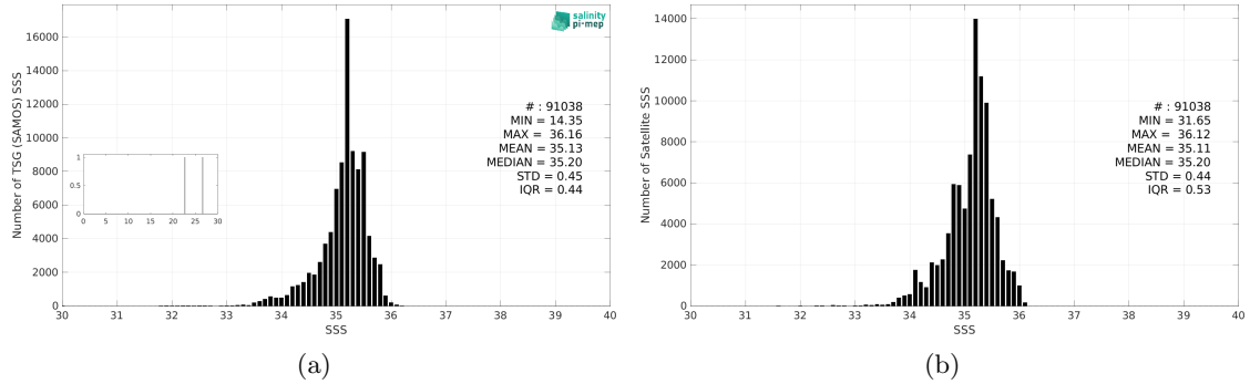
Figure 3: Histograms of SSS from TSG (SAMOS) (a) and SMAP SSS L3 v5.3 - Monthly (RSS) (b) considering all match-up pairs per bins of 0.1 over the South Pacific Ocean Pi-MEP region and for the full satellite product period.
