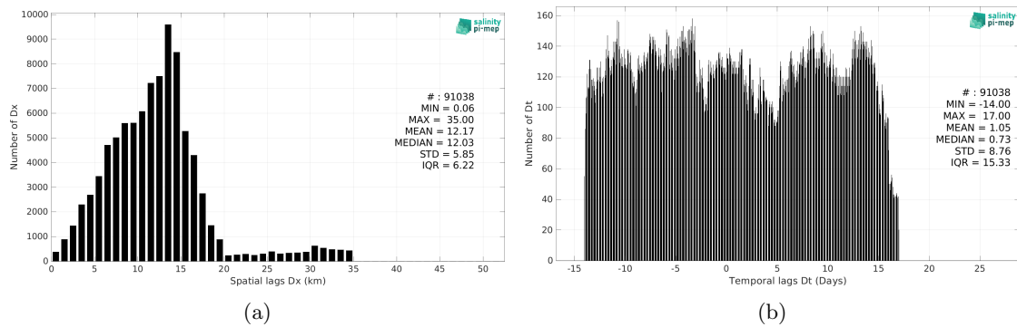
Figure 6: Histograms of the spatial (a) and temporal (b) lags between the location/time of the TSG (SAMOS) measurement and the date of the corresponding SMAP SSS L3 v5.3 - Monthly (RSS) SSS pixel.
