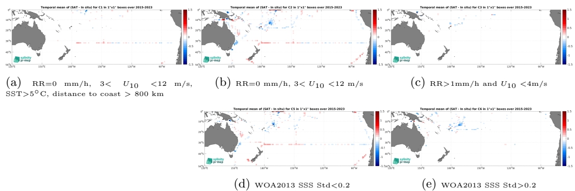
Figure 14: Temporal mean gridded over spatial boxes of size 1^\circ \times 1^\circ of \Delta\text{SSS} (SMAP SSS L3 v5.3 - Monthly (RSS) - TSG (SAMOS)) for 5 different subdatasets corresponding to:RR=0 mm/h, 3 < U_{10} < 12 m/s, SST >5^\circ\text{C} , distance to coast > 800 km (a), RR=0 mm/h, 3 < U_{10} < 12 m/s (b), RR >1 mm/h and U_{10} < 4 m/s (c), WOA2013 SSS Std <0.2 (d), WOA2013 SSS Std >0.2 (e).
