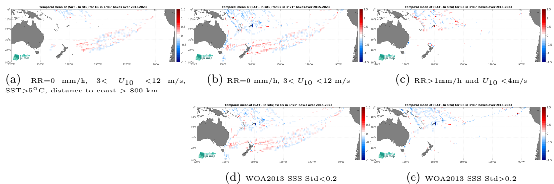
Figure 14: Temporal mean gridded over spatial boxes of size 1^\circ \times 1^\circ of \Delta\text{SSS} (SMAP SSS L3 v5.3 - Monthly (RSS) - TSG (LEGOS-DM)) for 5 different subdatasets corresponding to:RR=0 mm/h, 3 < U_{10} < 12 m/s, SST >5^\circ\text{C} , distance to coast > 800 km (a), RR=0 mm/h, 3 < U_{10} < 12 m/s (b), RR >1 mm/h and U_{10} < 4 m/s (c), WOA2013 SSS Std <0.2 (d), WOA2013 SSS Std >0.2 (e).
