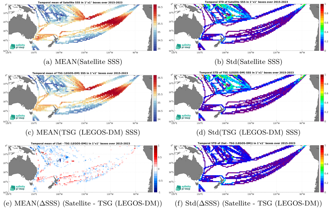
Figure 7: Temporal mean (left) and Std (right) of SSS from SMAP SSS L3 v5.3 - Monthly (RSS) (top), TSG (LEGOS-DM) (middle), and of \Delta\text{SSS} (Satellite - TSG (LEGOS-DM)). Only match-up pairs are used to generate these maps.
