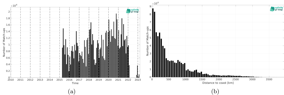
Figure 2: Number of match-ups between TSG (LEGOS-DM) and SMAP SSS L3 v5.3 - Monthly (RSS) SSS as a function of time (a) and as function of the distance to coast (b) over the South Pacific Ocean Pi-MEP region and for the full satellite product period.
