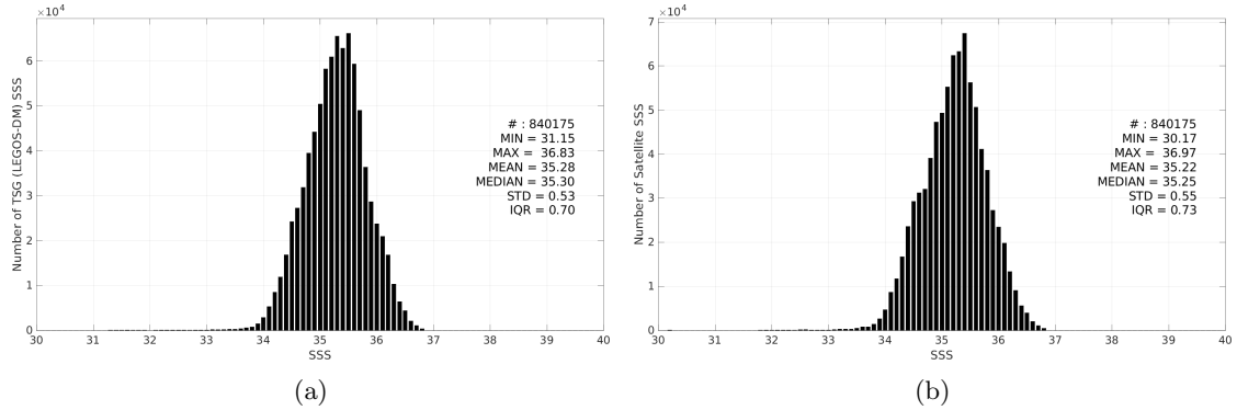
Figure 3: Histograms of SSS from TSG (LEGOS-DM) (a) and SMAP SSS L3 v5.3 - Monthly (RSS) (b) considering all match-up pairs per bins of 0.1 over the South Pacific Ocean Pi-MEP region and for the full satellite product period.
