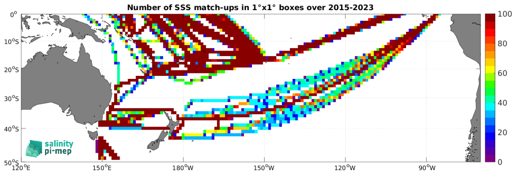
Figure 5: Number of SSS match-ups between TSG (LEGOS-DM) SSS and the SMAP SSS L3 v5.3 - Monthly (RSS) SSS product for the South Pacific Ocean Pi-MEP region over 1^\circ \times 1^\circ boxes and for the full satellite product period.
