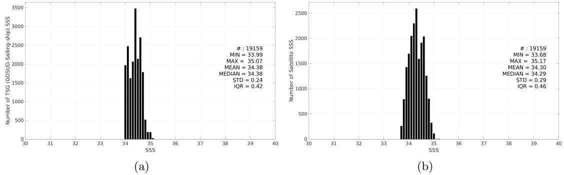
Figure 3: Histograms of SSS from TSG (GOSUD-Sailing-ship) (a) and SMAP SSS L3 v5.3 - Monthly (RSS) (b) considering all match-up pairs per bins of 0.1 over the South Pacific Ocean Pi-MEP region and for the full satellite product period.
