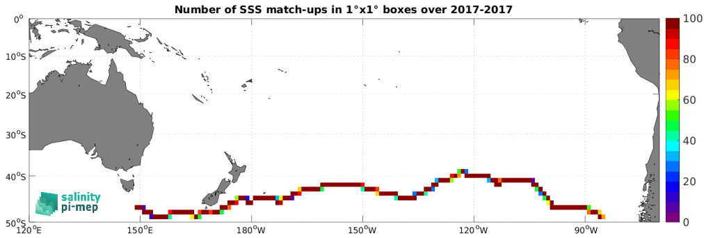
Figure 5: Number of SSS match-ups between TSG (GOSUD-Sailing-ship) SSS and the SMAP SSS L3 v5.3 - Monthly (RSS) SSS product for the South Pacific Ocean Pi-MEP region over 1^\circ \times 1^\circ boxes and for the full satellite product period.
