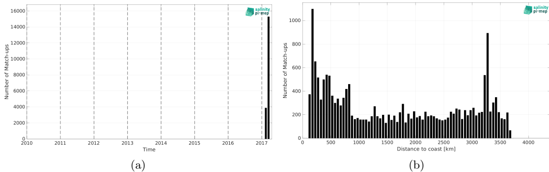
Figure 2: Number of match-ups between TSG (GOSUD-Sailing-ship) and SMAP SSS L3 v5.3 - Monthly (RSS) SSS as a function of time (a) and as function of the distance to coast (b) over the South Pacific Ocean Pi-MEP region and for the full satellite product period.
