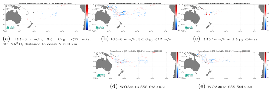
Figure 14: Temporal mean gridded over spatial boxes of size 1^\circ \times 1^\circ of \Delta SSS (SMAP SSS L3 v5.3 - Monthly (RSS) - TSG (GOSUD-Research-vessel)) for 5 different subdatasets corresponding to:RR=0 mm/h, 3 < U_{10} < 12 m/s, SST >5^\circ\text{C} , distance to coast > 800 km (a), RR=0 mm/h, 3 < U_{10} < 12 m/s (b), RR >1 mm/h and U_{10} < 4 m/s (c), WOA2013 SSS Std <0.2 (d), WOA2013 SSS Std >0.2 (e).
