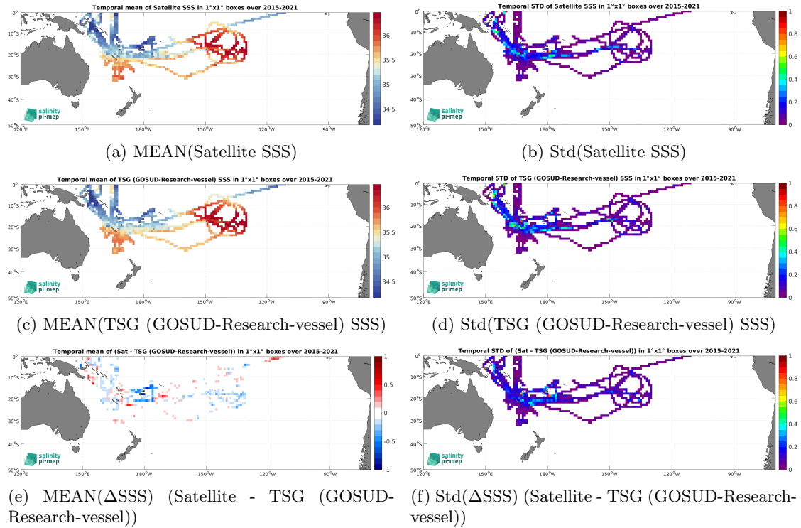
Figure 7: Temporal mean (left) and Std (right) of SSS from SMAP SSS L3 v5.3 - Monthly (RSS) (top), TSG (GOSUD-Research-vessel) (middle), and of \Delta SSS (Satellite - TSG (GOSUD-Research-vessel)). Only match-up pairs are used to generate these maps.
