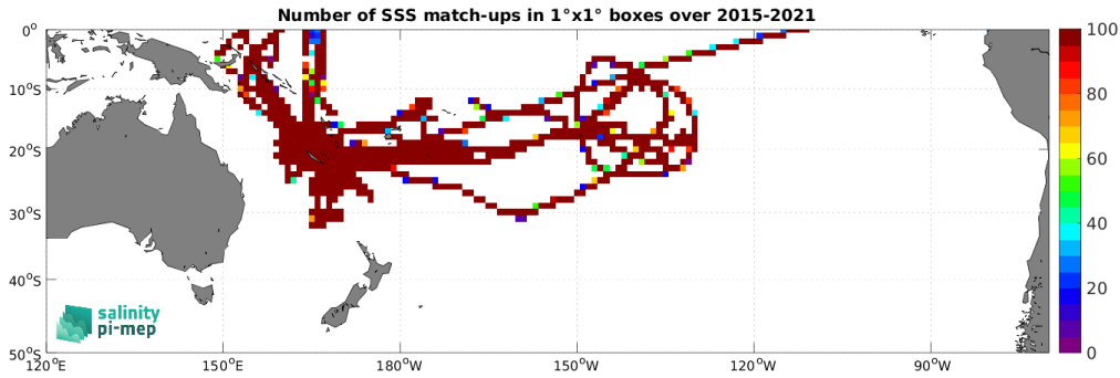
Figure 5: Number of SSS match-ups between TSG (GOSUD-Research-vessel) SSS and the SMAP SSS L3 v5.3 - Monthly (RSS) SSS product for the South Pacific Ocean Pi-MEP region over 1^\circ \times 1^\circ boxes and for the full satellite product period.
