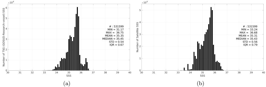
Figure 3: Histograms of SSS from TSG (GOSUD-Research-vessel) (a) and SMAP SSS L3 v5.3 - Monthly (RSS) (b) considering all match-up pairs per bins of 0.1 over the South Pacific Ocean Pi-MEP region and for the full satellite product period.
