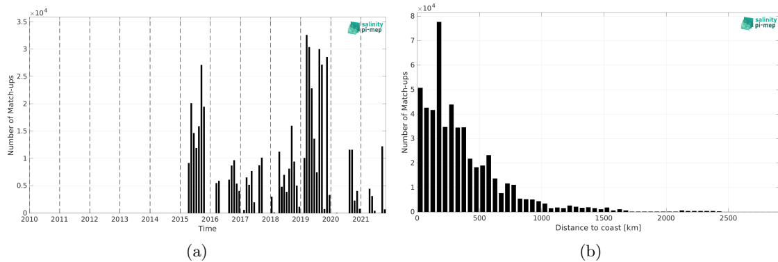
Figure 2: Number of match-ups between TSG (GOSUD-Research-vessel) and SMAP SSS L3 v5.3 - Monthly (RSS) SSS as a function of time (a) and as function of the distance to coast (b) over the South Pacific Ocean Pi-MEP region and for the full satellite product period.
