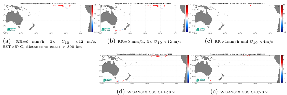
Figure 14: Temporal mean gridded over spatial boxes of size 1^\circ \times 1^\circ of \Delta\text{SSS} (SMAP SSS L3 v5.3 - Monthly (RSS) - Sairdrone) for 5 different subdatasets corresponding to:RR=0 mm/h, 3 < U_{10} < 12 m/s, SST >5^\circ\text{C} , distance to coast > 800 km (a), RR=0 mm/h, 3 < U_{10} < 12 m/s (b), RR >1 mm/h and U_{10} < 4 m/s (c), WOA2013 SSS Std <0.2 (d), WOA2013 SSS Std >0.2 (e).
