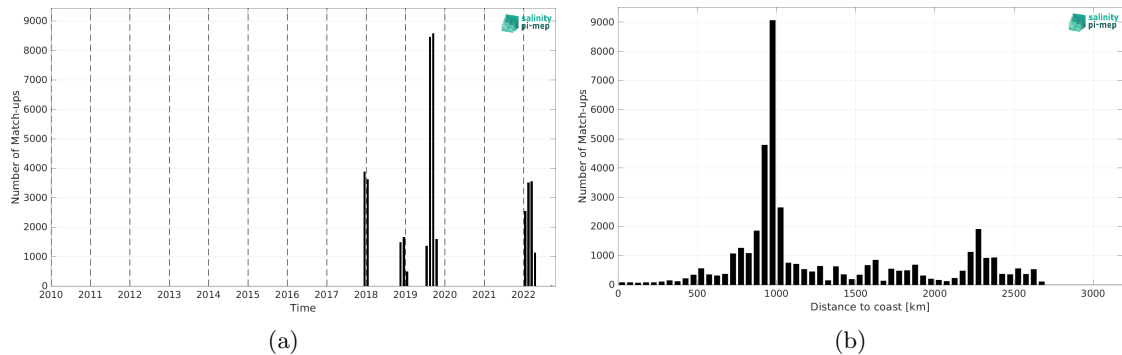
Figure 2: Number of match-ups between Saildrone and SMAP SSS L3 v5.3 - Monthly (RSS) SSS as a function of time (a) and as function of the distance to coast (b) over the South Pacific Ocean Pi-MEP region and for the full satellite product period.
