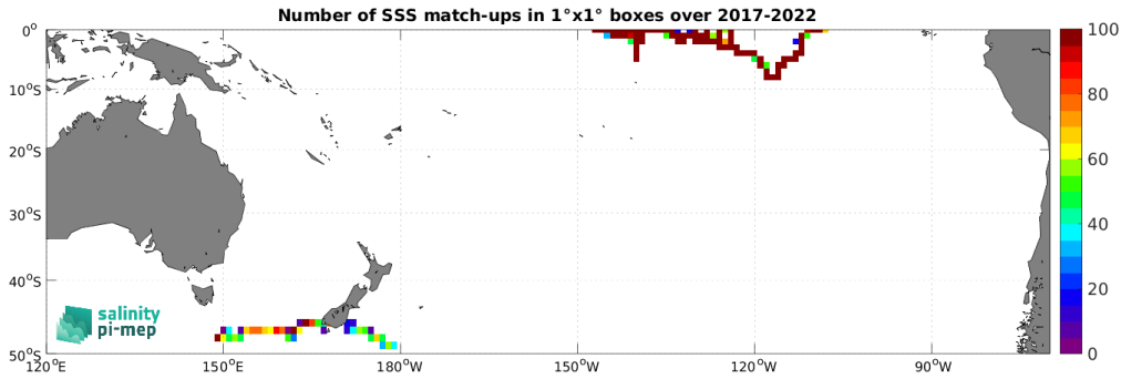
Figure 5: Number of SSS match-ups between Saildrone SSS and the SMAP SSS L3 v5.3 - Monthly (RSS) SSS product for the South Pacific Ocean Pi-MEP region over 1^\circ \times 1^\circ boxes and for the full satellite product period.
