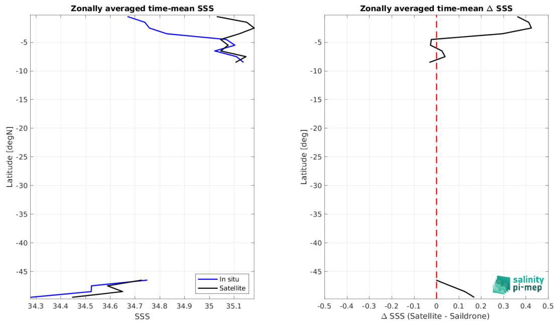
Figure 9: Left panel: Zonal mean SSS from SMAP SSS L3 v5.3 - Monthly (RSS) satellite product (black) and from Sairdrone (blue). Right panel: Zonal mean of \Delta SSS (Satellite - Sairdrone) for all the collected Pi-MEP match-up pairs estimated over the full satellite product period.
