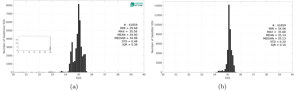
Figure 3: Histograms of SSS from Saildrone (a) and SMAP SSS L3 v5.3 - Monthly (RSS) (b) considering all match-up pairs per bins of 0.1 over the South Pacific Ocean Pi-MEP region and for the full satellite product period.
