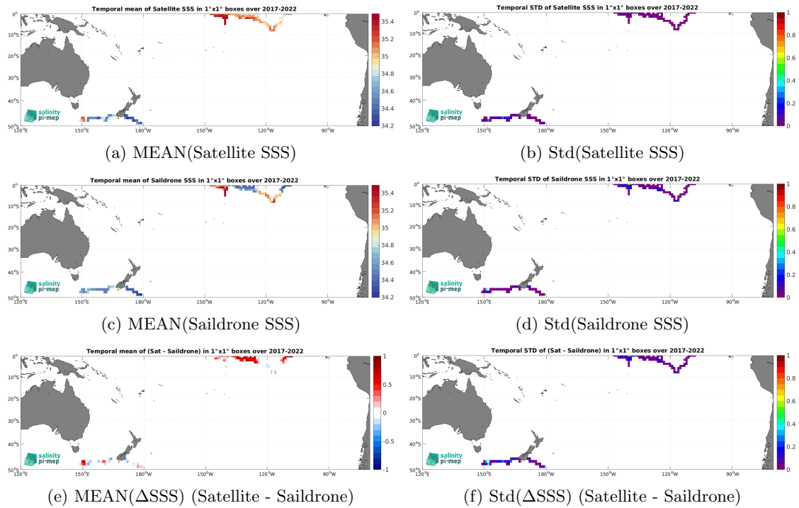
Figure 7: Temporal mean (left) and Std (right) of SSS from SMAP SSS L3 v5.3 - Monthly (RSS) (top), Saildrone (middle), and of \Delta SSS (Satellite - Saildrone). Only match-up pairs are used to generate these maps.
