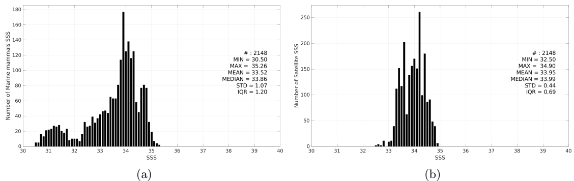
Figure 3: Histograms of SSS from Marine mammals (a) and SMAP SSS L3 v5.3 - Monthly (RSS) (b) considering all match-up pairs per bins of 0.1 over the South Pacific Ocean Pi-MEP region and for the full satellite product period.
