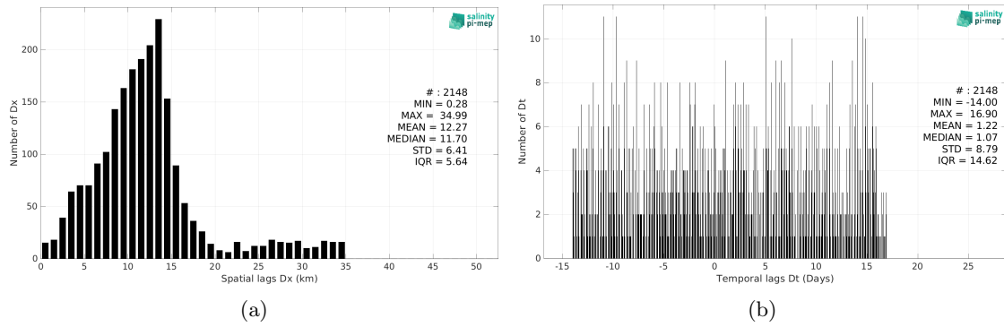
Figure 6: Histograms of the spatial (a) and temporal (b) lags between the location/time of the Marine mammals measurement and the date of the corresponding SMAP SSS L3 v5.3 - Monthly (RSS) SSS pixel.
