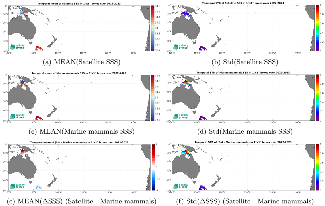
Figure 7: Temporal mean (left) and Std (right) of SSS from SMAP SSS L3 v5.3 - Monthly (RSS) (top), Marine mammals (middle), and of \Delta SSS (Satellite - Marine mammals). Only match-up pairs are used to generate these maps.
