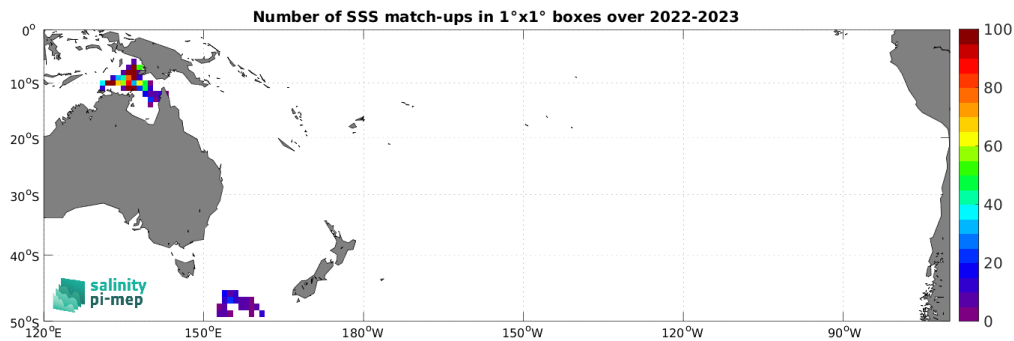
Figure 5: Number of SSS match-ups between Marine mammals SSS and the SMAP SSS L3 v5.3 - Monthly (RSS) SSS product for the South Pacific Ocean Pi-MEP region over 1^\circ \times 1^\circ boxes and for the full satellite product period.
