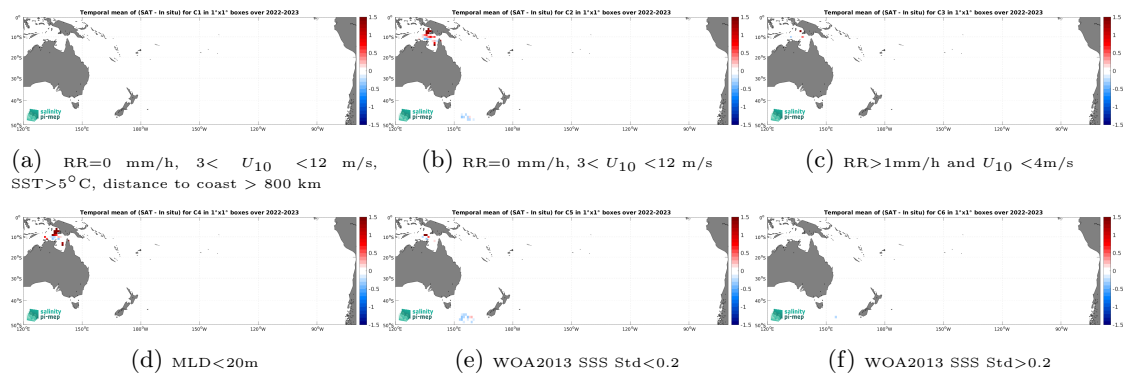
Figure 14: Temporal mean gridded over spatial boxes of size 1^\circ \times 1^\circ of \Delta SSS (SMAP SSS L3 v5.3 - Monthly (RSS) - Marine mammals) for 6 different subdatasets corresponding to:RR=0 mm/h, 3 < U_{10} < 12 m/s, SST>5°C, distance to coast > 800 km (a), RR=0 mm/h, 3 < U_{10} < 12 m/s (b), RR>1mm/h and U_{10} < 4 m/s (c),MLD<20m (d),WOA2013 SSS Std<0.2 (e),WOA2013 SSS Std>0.2 (f).
