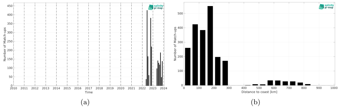
Figure 2: Number of match-ups between Marine mammals and SMAP SSS L3 v5.3 - Monthly (RSS) SSS as a function of time (a) and as function of the distance to coast (b) over the South Pacific Ocean Pi-MEP region and for the full satellite product period.
