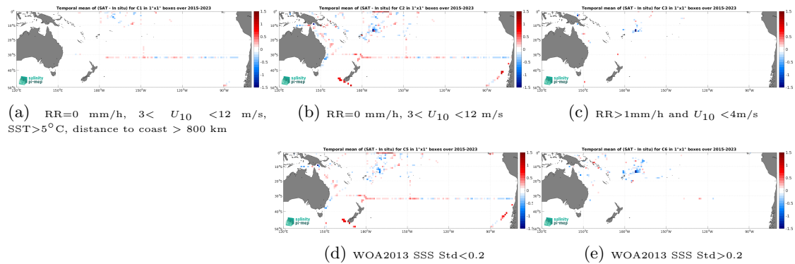
Figure 12: Temporal mean gridded over spatial boxes of size 1^\circ \times 1^\circ of \Delta\text{SSS} (SMAP SSS L3 v5 - 8-Day running (RSS) - TSG (SAMOS)) for 5 different subdatasets corresponding to:RR=0 mm/h, 3 < U_{10} < 12 m/s, SST >5^\circ\text{C} , distance to coast > 800 km (a), RR=0 mm/h, 3 < U_{10} < 12 m/s (b), RR >1 mm/h and U_{10} < 4 m/s (c), WOA2013 SSS Std <0.2 (d), WOA2013 SSS Std >0.2 (e).
