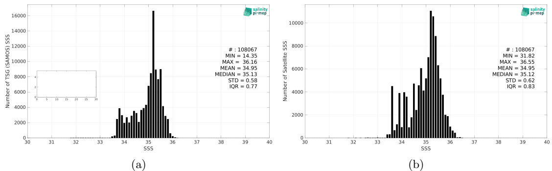
Figure 2: Histograms of SSS from TSG (SAMOS) (a) and SMAP SSS L3 v5 - 8-Day running (RSS) (b) considering all match-up pairs per bins of 0.1 over the South Pacific Ocean Pi-MEP region and for the full satellite product period.
