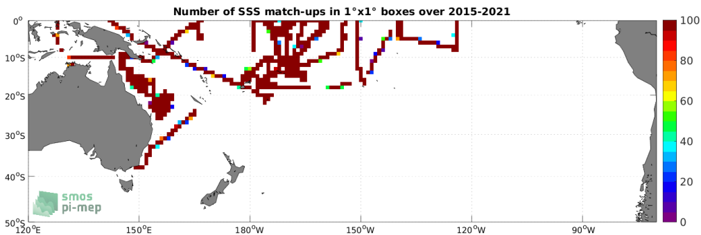
Figure 4: Number of SSS match-ups between TSG (SAMOS) SSS and the SMAP SSS L3 v5 - 8-Day running (RSS) SSS product for the South Pacific Ocean Pi-MEP region over 1^\circ \times 1^\circ boxes and for the full satellite product period.
