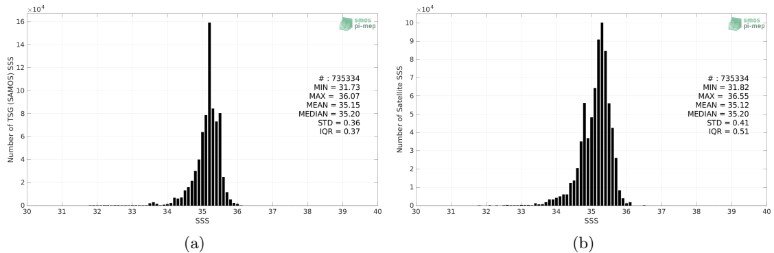
Figure 2: Histograms of SSS from TSG (SAMOS) (a) and SMAP SSS L3 v5 - 8-Day running (RSS) (b) considering all match-up pairs per bins of 0.1 over the South Pacific Ocean Pi-MEP region and for the full satellite product period.
