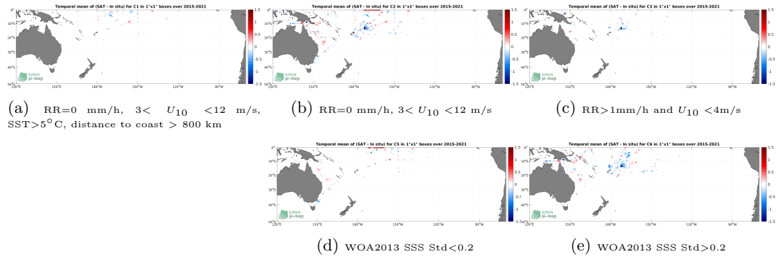
Figure 12: Temporal mean gridded over spatial boxes of size 1^\circ \times 1^\circ of \Delta SSS (SMAP SSS L3 v5 - 8-Day running (RSS) - TSG (SAMOS)) for 5 different subdatasets corresponding to:RR=0 mm/h, 3 < U_{10} < 12 m/s, SST > 5^\circ\text{C} , distance to coast > 800 km (a), RR=0 mm/h, 3 < U_{10} < 12 m/s (b), RR > 1 mm/h and U_{10} < 4 m/s (c), WOA2013 SSS Std < 0.2 (d), WOA2013 SSS Std > 0.2 (e).
