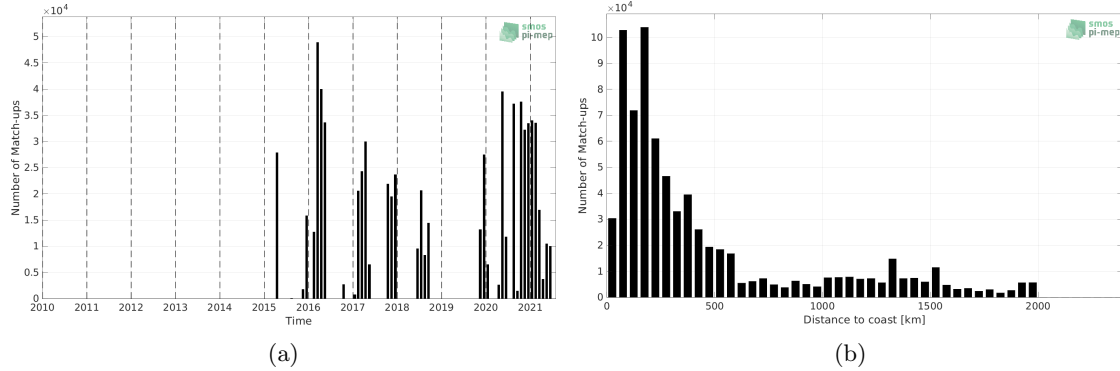
Figure 1: Number of match-ups between TSG (SAMOS) and SMAP SSS L3 v5 - 8-Day running (RSS) SSS as a function of time (a) and as function of the distance to coast (b) over the South Pacific Ocean Pi-MEP region and for the full satellite product period.
