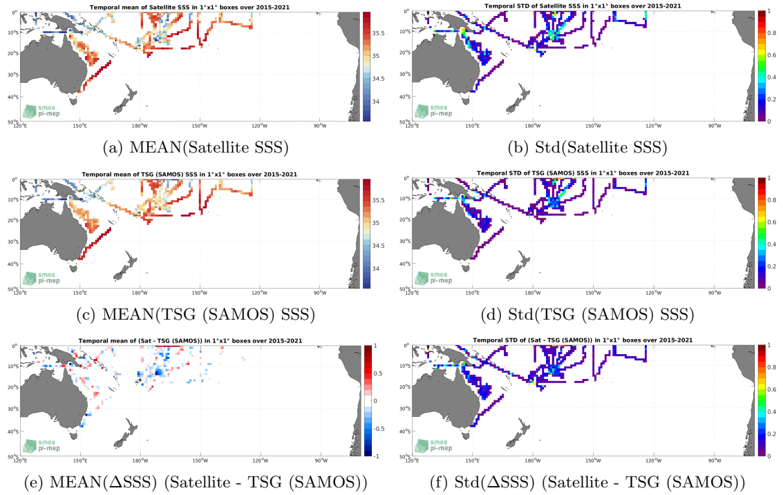
Figure 6: Temporal mean (left) and Std (right) of SSS from SMAP SSS L3 v5 - 8-Day running (RSS) (top), TSG (SAMOS) (middle), and of \Delta SSS (Satellite - TSG (SAMOS)). Only match-up pairs are used to generate these maps.
