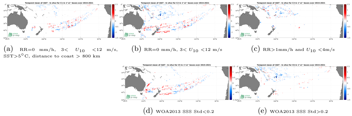
Figure 12: Temporal mean gridded over spatial boxes of size 1^\circ \times 1^\circ of \Delta SSS (SMAP SSS L3 v5 - 8-Day running (RSS) - TSG (LEGOS-DM)) for 5 different subdatasets corresponding to:RR=0 mm/h, 3 < U_{10} < 12 m/s, SST >5^\circ C, distance to coast > 800 km (a), RR=0 mm/h, 3 < U_{10} < 12 m/s (b), RR >1 mm/h and U_{10} < 4 m/s (c), WOA2013 SSS Std <0.2 (d), WOA2013 SSS Std >0.2 (e).
