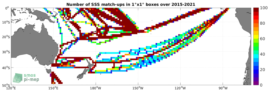
Figure 4: Number of SSS match-ups between TSG (LEGOS-DM) SSS and the SMAP SSS L3 v5 - 8-Day running (RSS) SSS product for the South Pacific Ocean Pi-MEP region over 1^\circ \times 1^\circ boxes and for the full satellite product period.
