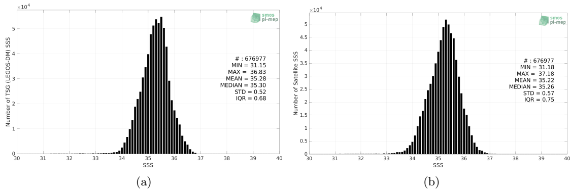
Figure 2: Histograms of SSS from TSG (LEGOS-DM) (a) and SMAP SSS L3 v5 - 8-Day running (RSS) (b) considering all match-up pairs per bins of 0.1 over the South Pacific Ocean Pi-MEP region and for the full satellite product period.
