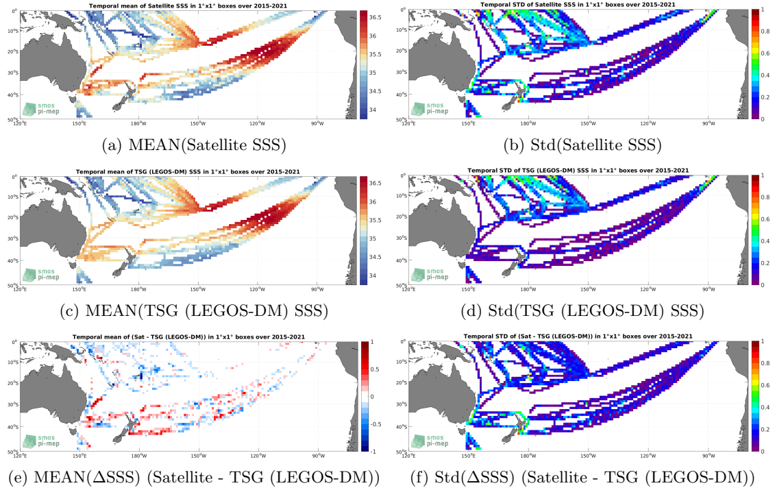
Figure 6: Temporal mean (left) and Std (right) of SSS from SMAP SSS L3 v5 - 8-Day running (RSS) (top), TSG (LEGOS-DM) (middle), and of \Delta SSS (Satellite - TSG (LEGOS-DM)). Only match-up pairs are used to generate these maps.
