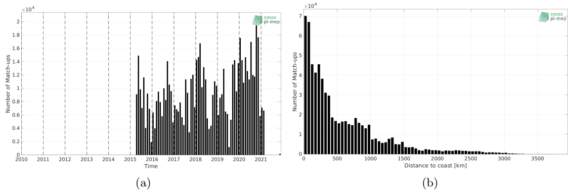
Figure 1: Number of match-ups between TSG (LEGOS-DM) and SMAP SSS L3 v5 - 8-Day running (RSS) SSS as a function of time (a) and as function of the distance to coast (b) over the South Pacific Ocean Pi-MEP region and for the full satellite product period.
