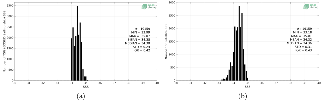
Figure 2: Histograms of SSS from TSG (GOSUD-Sailing-ship) (a) and SMAP SSS L3 v5 - 8-Day running (RSS) (b) considering all match-up pairs per bins of 0.1 over the South Pacific Ocean Pi-MEP region and for the full satellite product period.
