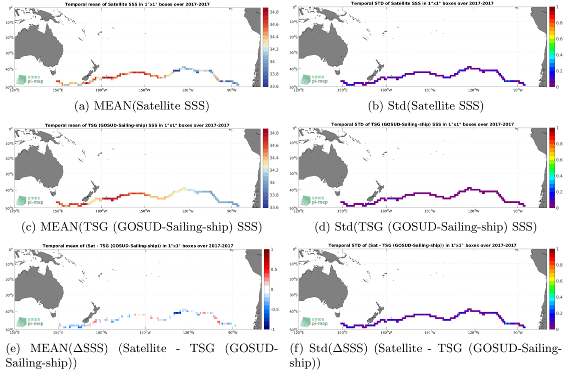
Figure 6: Temporal mean (left) and Std (right) of SSS from SMAP SSS L3 v5 - 8-Day running (RSS) (top), TSG (GOSUD-Sailing-ship) (middle), and of \Delta SSS (Satellite - TSG (GOSUD-Sailing-ship)). Only match-up pairs are used to generate these maps.
