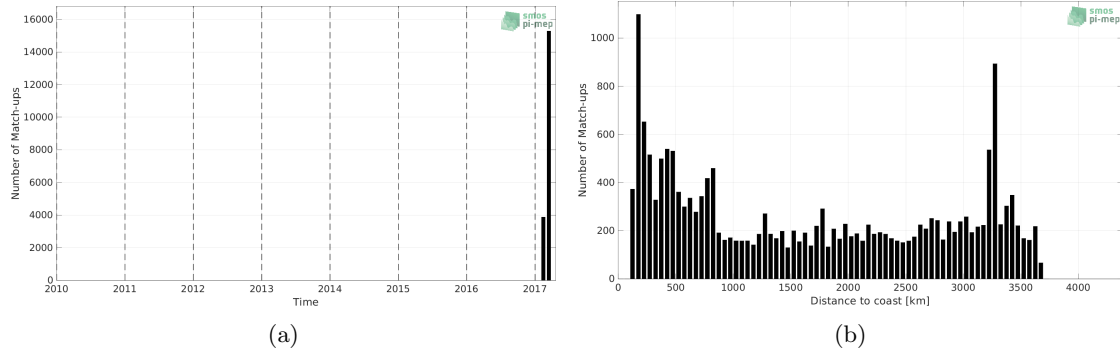
Figure 1: Number of match-ups between TSG (GOSUD-Sailing-ship) and SMAP SSS L3 v5 - 8-Day running (RSS) SSS as a function of time (a) and as function of the distance to coast (b) over the South Pacific Ocean Pi-MEP region and for the full satellite product period.
