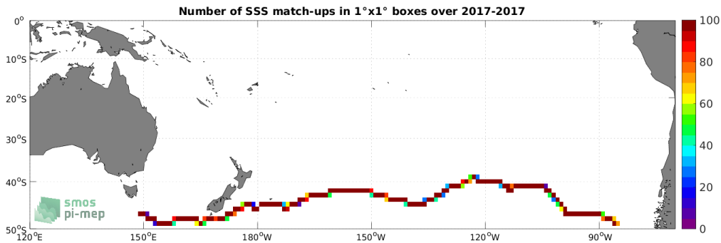
Figure 4: Number of SSS match-ups between TSG (GOSUD-Sailing-ship) SSS and the SMAP SSS L3 v5 - 8-Day running (RSS) SSS product for the South Pacific Ocean Pi-MEP region over 1^\circ \times 1^\circ boxes and for the full satellite product period.
