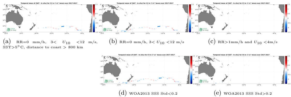
Figure 12: Temporal mean gridded over spatial boxes of size 1^\circ \times 1^\circ of \Delta SSS (SMAP SSS L3 v5 - 8-Day running (RSS) - TSG (GOSUD-Sailing-ship)) for 5 different subdatasets corresponding to:RR=0 mm/h, 3 < U_{10} < 12 m/s, SST >5^\circ\text{C} , distance to coast > 800 km (a), RR=0 mm/h, 3 < U_{10} < 12 m/s (b), RR >1 mm/h and U_{10} < 4 m/s (c), WOA2013 SSS Std <0.2 (d), WOA2013 SSS Std >0.2 (e).
