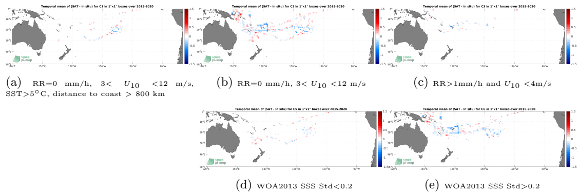
Figure 12: Temporal mean gridded over spatial boxes of size 1^\circ \times 1^\circ of \Delta SSS (SMAP SSS L3 v5 - 8-Day running (RSS) - TSG (GOSUD-Research-vessel)) for 5 different subdatasets corresponding to:RR=0 mm/h, 3 < U_{10} < 12 m/s, SST >5^\circ\text{C} , distance to coast > 800 km (a), RR=0 mm/h, 3 < U_{10} < 12 m/s (b), RR >1 mm/h and U_{10} < 4 m/s (c), WOA2013 SSS Std <0.2 (d), WOA2013 SSS Std >0.2 (e).
