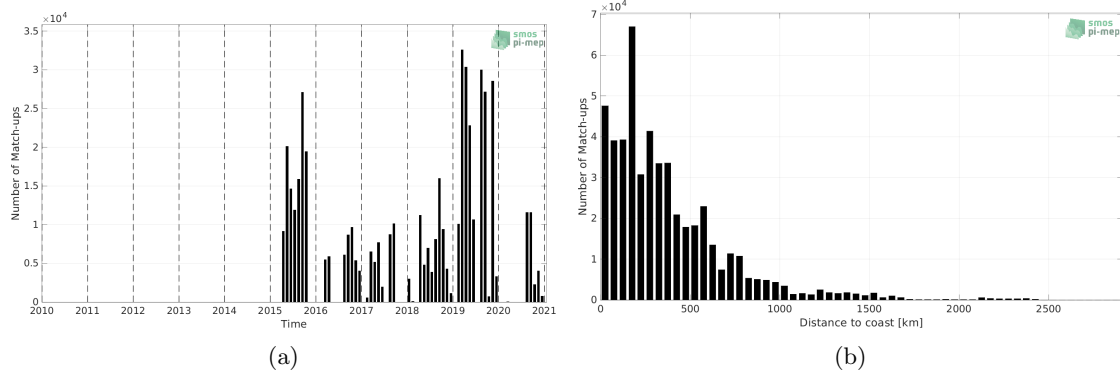
Figure 1: Number of match-ups between TSG (GOSUD-Research-vessel) and SMAP SSS L3 v5 - 8-Day running (RSS) SSS as a function of time (a) and as function of the distance to coast (b) over the South Pacific Ocean Pi-MEP region and for the full satellite product period.
