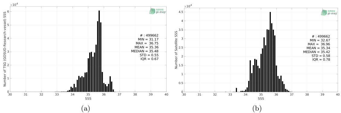
Figure 2: Histograms of SSS from TSG (GOSUD-Research-vessel) (a) and SMAP SSS L3 v5 - 8-Day running (RSS) (b) considering all match-up pairs per bins of 0.1 over the South Pacific Ocean Pi-MEP region and for the full satellite product period.
