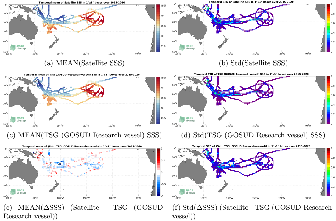
Figure 6: Temporal mean (left) and Std (right) of SSS from SMAP SSS L3 v5 - 8-Day running (RSS) (top), TSG (GOSUD-Research-vessel) (middle), and of \Delta SSS (Satellite - TSG (GOSUD-Research-vessel)). Only match-up pairs are used to generate these maps.
