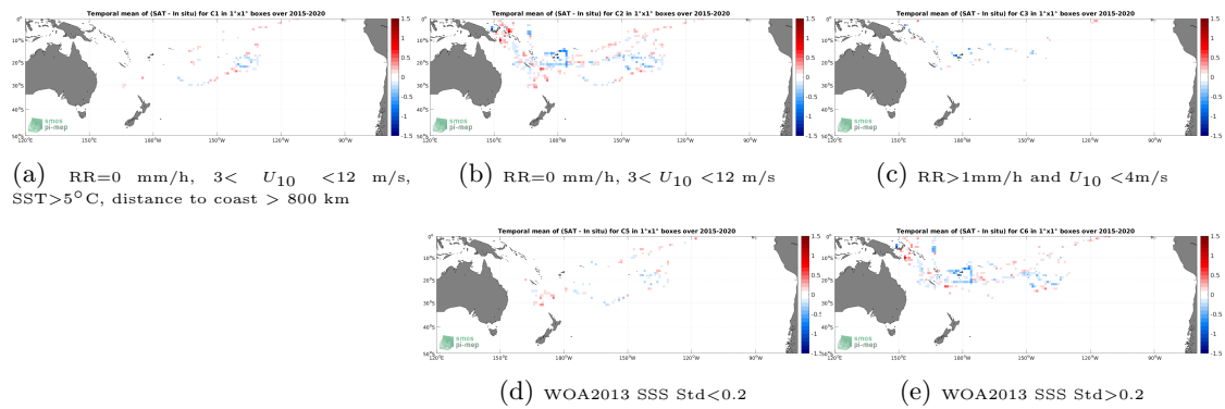
Figure 12: Temporal mean gridded over spatial boxes of size 1^\circ \times 1^\circ of \Delta\text{SSS} (SMAP SSS L3 v5 - 8-Day running (RSS) - TSG (GOSUD-Research-vessel)) for 5 different subdatasets corresponding to:RR=0 mm/h, 3 < U_{10} < 12 m/s, SST>5°C, distance to coast > 800 km (a), RR=0 mm/h, 3 < U_{10} < 12 m/s (b), RR>1mm/h and U_{10} < 4 m/s (c), WOA2013 SSS Std<0.2 (d), WOA2013 SSS Std>0.2 (e).
