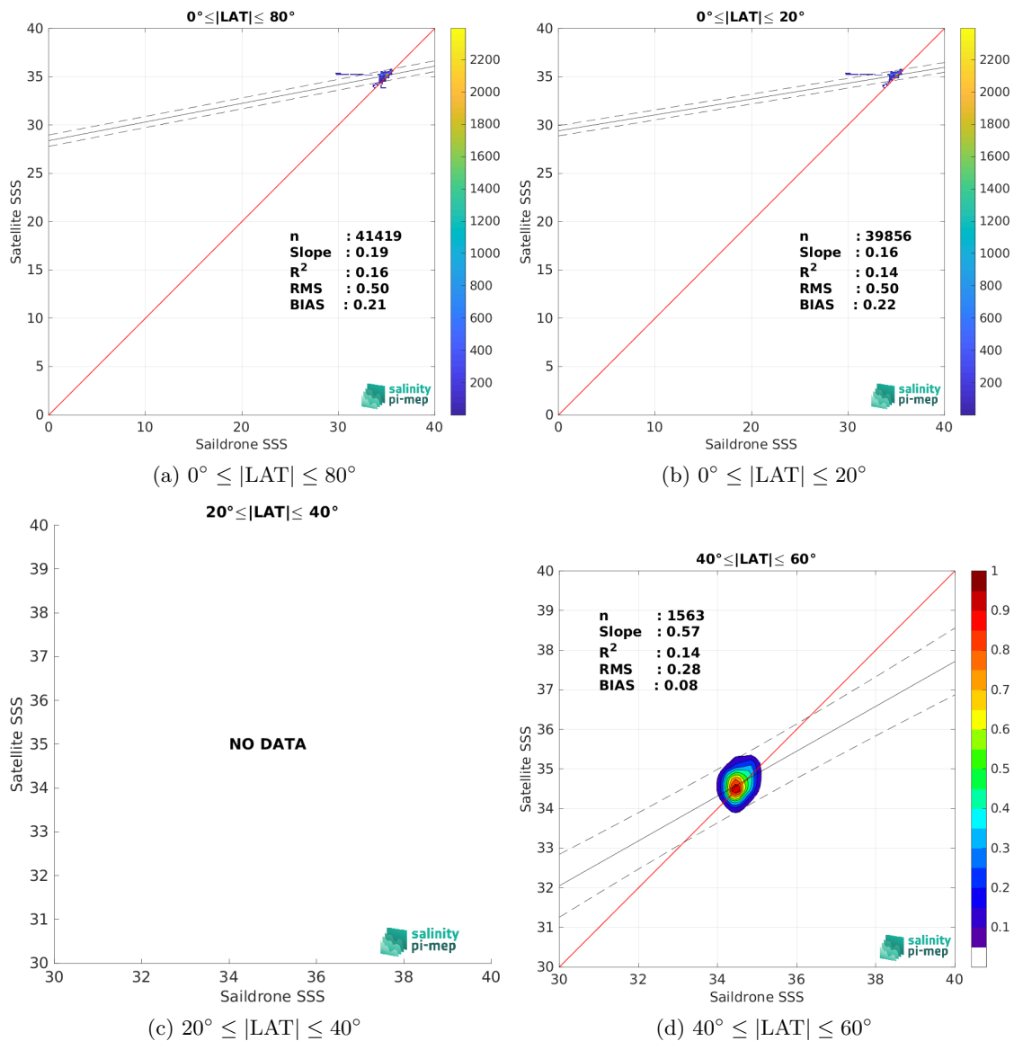
Figure 9: Contour maps of the concentration of SMAP SSS L3 v5 - 8-Day running (RSS) SSS (y-axis) versus Sairdrone SSS (x-axis) at match-up pairs for different latitude bands. For each plot, the red line shows x=y . The black thin and dashed lines indicate a linear fit through the data cloud and the \pm 95\% confidence levels, respectively. The number match-up pairs n , the slope and R^2 coefficient of the linear fit, the root mean square (RMS) and the mean bias between satellite and in situ data are indicated for each latitude band in each plots.
