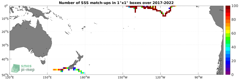
Figure 4: Number of SSS match-ups between Saildrone SSS and the SMAP SSS L3 v5 - 8-Day running (RSS) SSS product for the South Pacific Ocean Pi-MEP region over 1^\circ \times 1^\circ boxes and for the full satellite product period.
