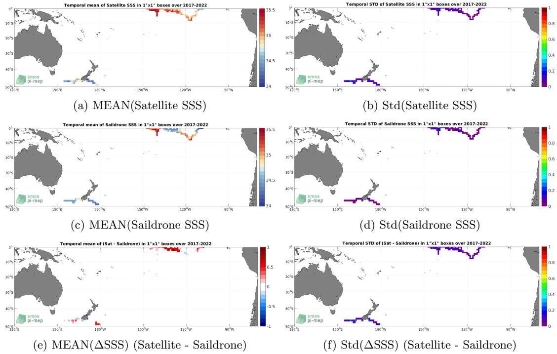
Figure 6: Temporal mean (left) and Std (right) of SSS from SMAP SSS L3 v5 - 8-Day running (RSS) (top), Saildrone (middle), and of \Delta SSS (Satellite - Saildrone). Only match-up pairs are used to generate these maps.
