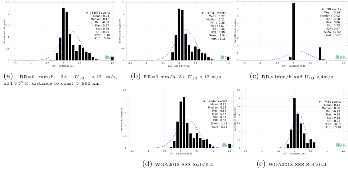
Figure 13: Normalized histogram of \Delta SSS (SMAP SSS L3 v5 - 8-Day running (RSS) - Saldrone) for 5 different subdatasets corresponding to: RR=0 mm/h, 3 < U_{10} < 12 m/s, SST > 5°C, distance to coast > 800 km (a), RR=0 mm/h, 3 < U_{10} < 12 m/s (b), RR > 1mm/h and U_{10} < 4 m/s (c), WOA2013 SSS Std < 0.2 (d), WOA2013 SSS Std > 0.2 (e).
