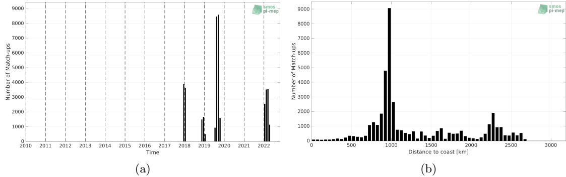
Figure 1: Number of match-ups between Saildrone and SMAP SSS L3 v5 - 8-Day running (RSS) SSS as a function of time (a) and as function of the distance to coast (b) over the South Pacific Ocean Pi-MEP region and for the full satellite product period.
