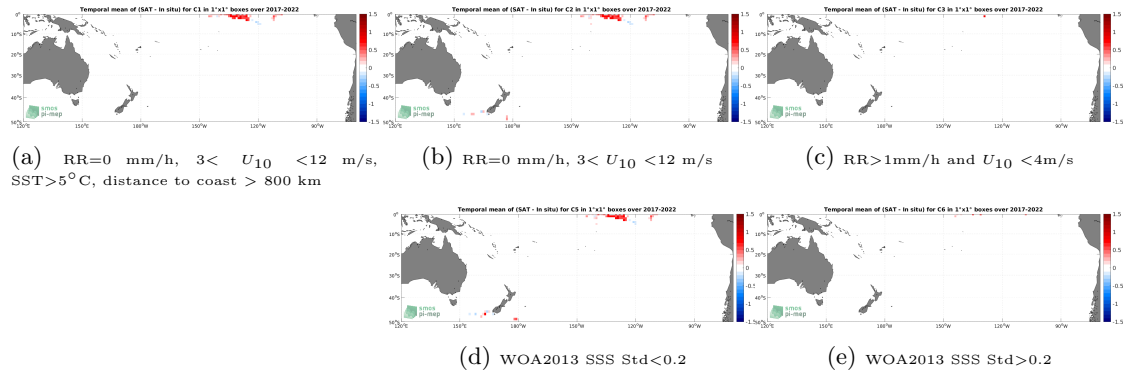
Figure 12: Temporal mean gridded over spatial boxes of size 1^\circ \times 1^\circ of \Delta SSS (SMAP SSS L3 v5 - 8-Day running (RSS) - Saildrone) for 5 different subdatasets corresponding to:RR=0 mm/h, 3 < U_{10} < 12 m/s, SST >5^\circ\text{C} , distance to coast > 800 km (a), RR=0 mm/h, 3 < U_{10} < 12 m/s (b), RR >1 mm/h and U_{10} < 4 m/s (c), WOA2013 SSS Std <0.2 (d), WOA2013 SSS Std >0.2 (e).
