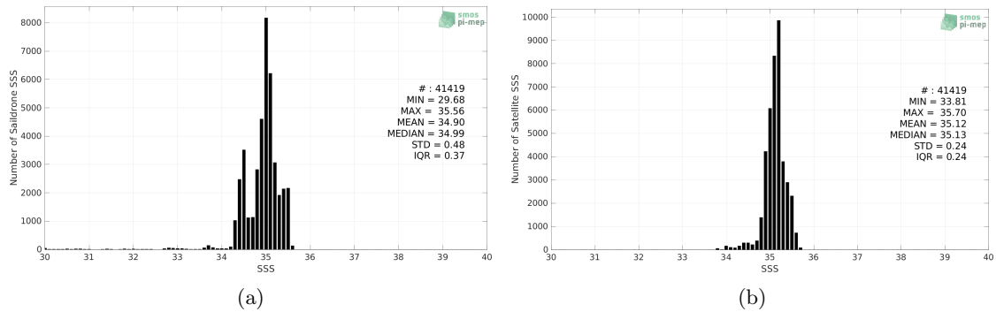
Figure 2: Histograms of SSS from Saildrone (a) and SMAP SSS L3 v5 - 8-Day running (RSS) (b) considering all match-up pairs per bins of 0.1 over the South Pacific Ocean Pi-MEP region and for the full satellite product period.
