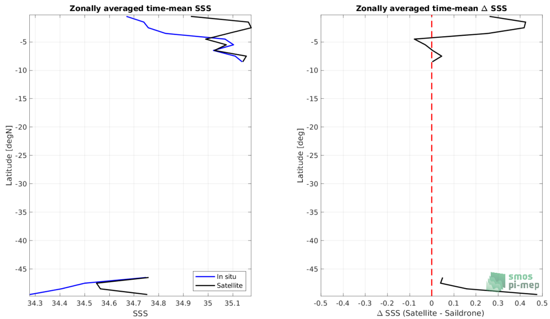
Figure 8: Left panel: Zonal mean SSS from SMAP SSS L3 v5 - 8-Day running (RSS) satellite product (black) and from Saildrone (blue). Right panel: Zonal mean of \Delta SSS (Satellite - Saildrone) for all the collected Pi-MEP match-up pairs estimated over the full satellite product period.
