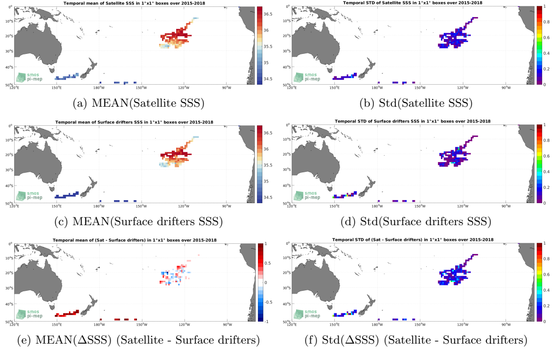
Figure 5: Temporal mean (left) and Std (right) of SSS from SMAP SSS L3 v5 - 8-Day running (RSS) (top), Surface drifters (middle), and of \Delta\text{SSS} (Satellite - Surface drifters). Only match-up pairs are used to generate these maps.
