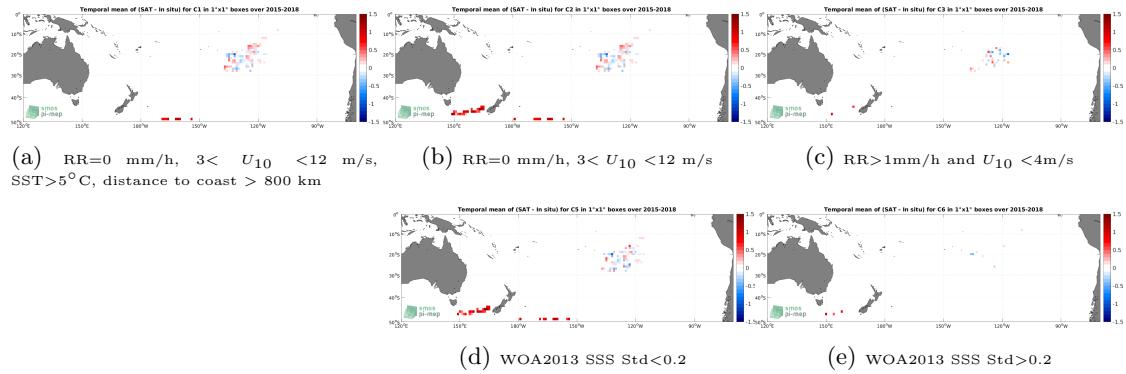
Figure 11: Temporal mean gridded over spatial boxes of size 1^\circ \times 1^\circ of \Delta\text{SSS} (SMAP SSS L3 v5 - 8-Day running (RSS) - Surface drifters) for 5 different subdatasets corresponding to:RR=0 mm/h, 3 < U_{10} < 12 m/s, SST > 5^\circ\text{C} , distance to coast > 800 km (a), RR=0 mm/h, 3 < U_{10} < 12 m/s (b), RR > 1 mm/h and U_{10} < 4 m/s (c), WOA2013 SSS Std < 0.2 (d), WOA2013 SSS Std > 0.2 (e).
