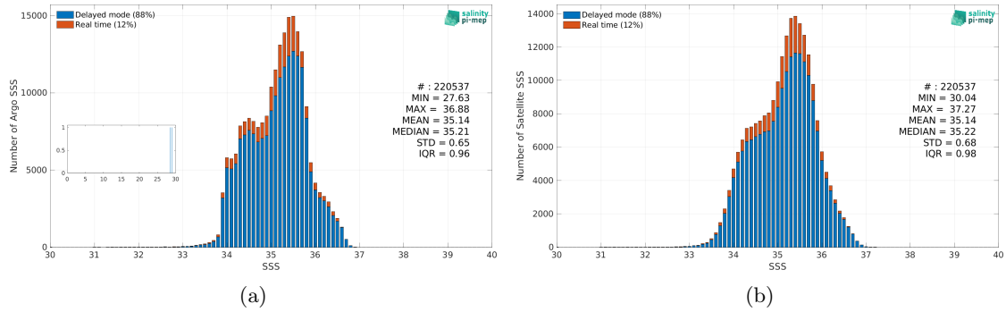
Figure 2: Histograms of SSS from Argo (a) and SMAP SSS L3 v5 - 8-Day running (RSS) (b) considering all match-up pairs per bins of 0.1 over the South Pacific Ocean Pi-MEP region and for the full satellite product period.
