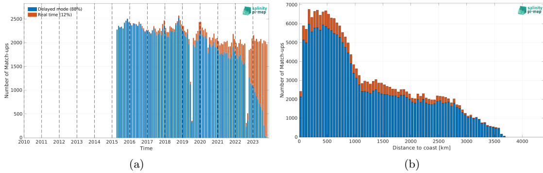
Figure 1: Number of match-ups between Argo and SMAP SSS L3 v5 - 8-Day running (RSS) SSS as a function of time (a) and as function of the distance to coast (b) over the South Pacific Ocean Pi-MEP region and for the full satellite product period.
