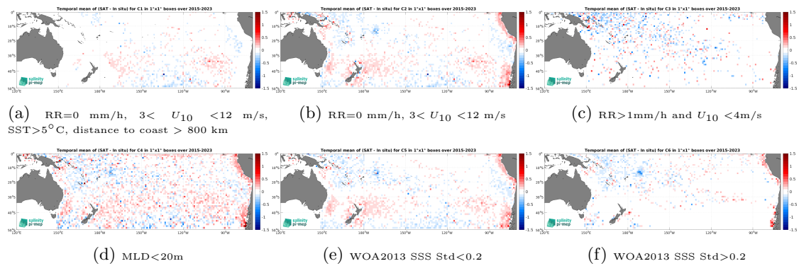
Figure 12: Temporal mean gridded over spatial boxes of size 1^\circ \times 1^\circ of \Delta SSS (SMAP SSS L3 v5 - 8-Day running (RSS) - Argo) for 6 different subdatasets corresponding to:RR=0 mm/h, 3 < U_{10} < 12 m/s, SST > 5^\circ\text{C} , distance to coast > 800 km (a), RR=0 mm/h, 3 < U_{10} < 12 m/s (b), RR > 1 mm/h and U_{10} < 4 m/s (c),MLD < 20 m (d),WOA2013 SSS Std < 0.2 (e),WOA2013 SSS Std > 0.2 (f).
