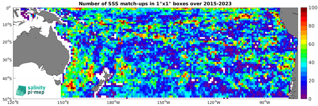
Figure 4: Number of SSS match-ups between Argo SSS and the SMAP SSS L3 v5 - 8-Day running (RSS) SSS product for the South Pacific Ocean Pi-MEP region over 1^\circ \times 1^\circ boxes and for the full satellite product period.
