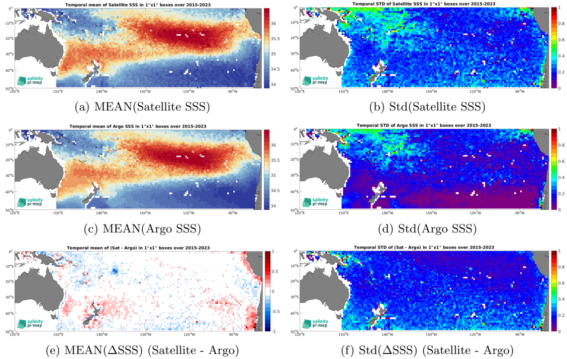
Figure 6: Temporal mean (left) and Std (right) of SSS from SMAP SSS L3 v5 - 8-Day running (RSS) (top), Argo (middle), and of \Delta SSS (Satellite - Argo). Only match-up pairs are used to generate these maps.
