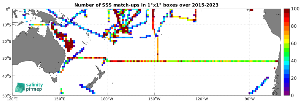
Figure 4: Number of SSS match-ups between TSG (SAMOS) SSS and the SMAP SSS L3 v5 - Monthly (RSS) SSS product for the South Pacific Ocean Pi-MEP region over 1^\circ \times 1^\circ boxes and for the full satellite product period.
