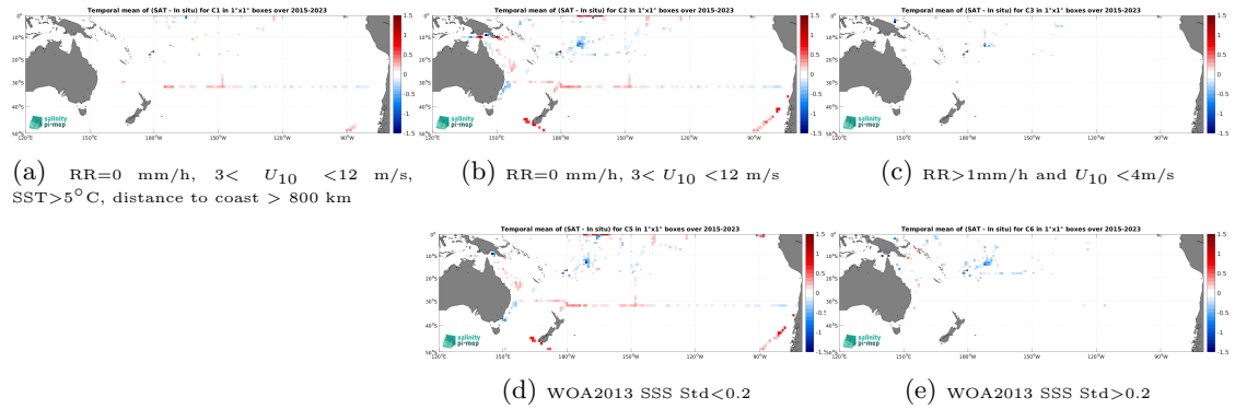
Figure 12: Temporal mean gridded over spatial boxes of size 1^\circ \times 1^\circ of \Delta SSS (SMAP SSS L3 v5 - Monthly (RSS) - TSG (SAMOS)) for 5 different subdatasets corresponding to:RR=0 mm/h, 3 < U_{10} < 12 m/s, SST >5^\circ C, distance to coast > 800 km (a), RR=0 mm/h, 3 < U_{10} < 12 m/s (b), RR >1 mm/h and U_{10} < 4 m/s (c), WOA2013 SSS Std <0.2 (d), WOA2013 SSS Std >0.2 (e).
