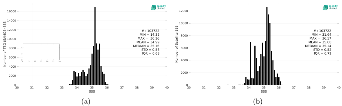
Figure 2: Histograms of SSS from TSG (SAMOS) (a) and SMAP SSS L3 v5 - Monthly (RSS) (b) considering all match-up pairs per bins of 0.1 over the South Pacific Ocean Pi-MEP region and for the full satellite product period.
