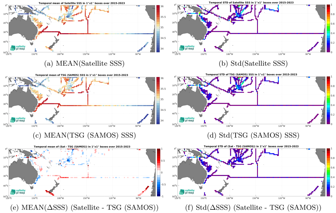
Figure 6: Temporal mean (left) and Std (right) of SSS from SMAP SSS L3 v5 - Monthly (RSS) (top), TSG (SAMOS) (middle), and of \Delta SSS (Satellite - TSG (SAMOS)). Only match-up pairs are used to generate these maps.
