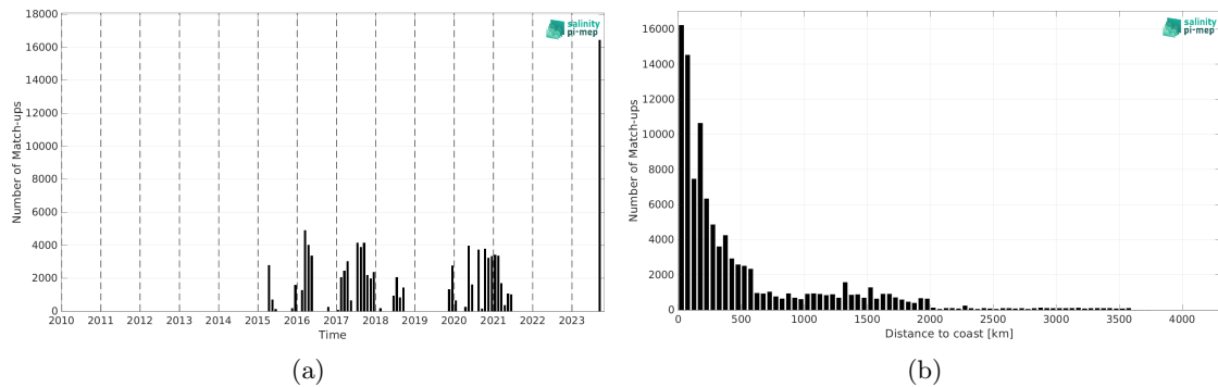
Figure 1: Number of match-ups between TSG (SAMOS) and SMAP SSS L3 v5 - Monthly (RSS) SSS as a function of time (a) and as function of the distance to coast (b) over the South Pacific Ocean Pi-MEP region and for the full satellite product period.
