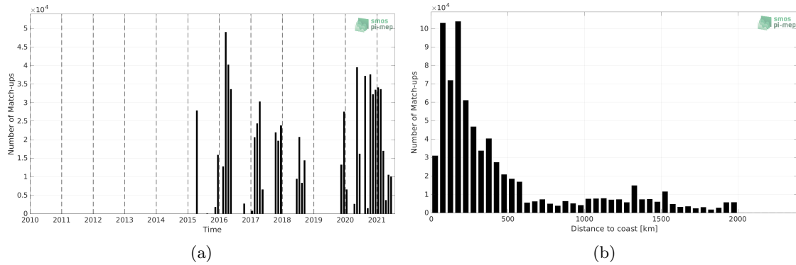
Figure 1: Number of match-ups between TSG (SAMOS) and SMAP SSS L3 v5 - Monthly (RSS) SSS as a function of time (a) and as function of the distance to coast (b) over the South Pacific Ocean Pi-MEP region and for the full satellite product period.
