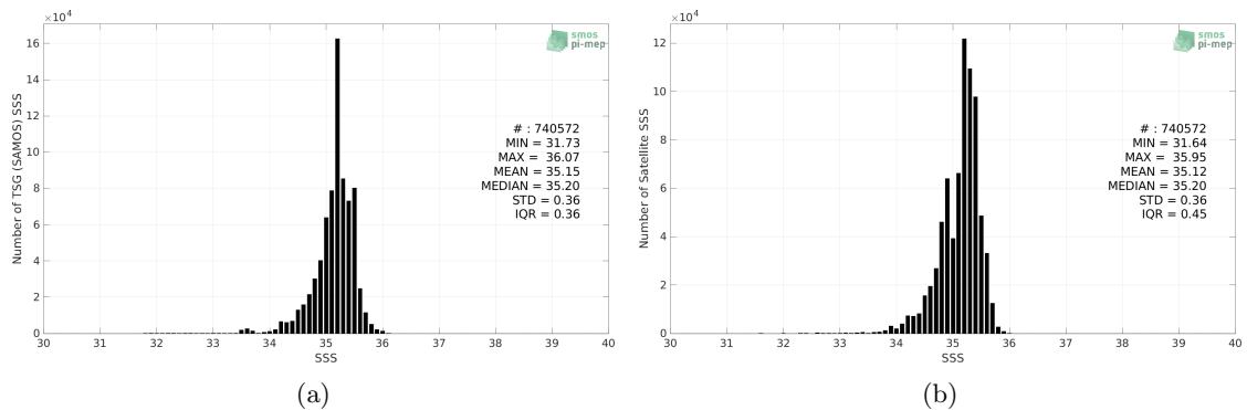
Figure 2: Histograms of SSS from TSG (SAMOS) (a) and SMAP SSS L3 v5 - Monthly (RSS) (b) considering all match-up pairs per bins of 0.1 over the South Pacific Ocean Pi-MEP region and for the full satellite product period.
