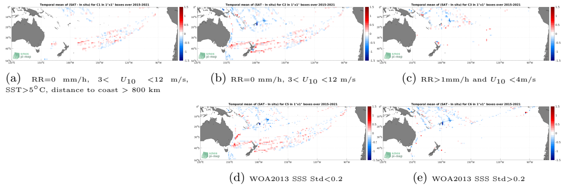
Figure 12: Temporal mean gridded over spatial boxes of size 1^\circ \times 1^\circ of \Delta SSS (SMAP SSS L3 v5 - Monthly (RSS) - TSG (LEGOS-DM)) for 5 different subdatasets corresponding to:RR=0 mm/h, 3 < U_{10} < 12 m/s, SST >5^\circ C, distance to coast > 800 km (a), RR=0 mm/h, 3 < U_{10} < 12 m/s (b), RR >1 mm/h and U_{10} < 4 m/s (c), WOA2013 SSS Std <0.2 (d), WOA2013 SSS Std >0.2 (e).
