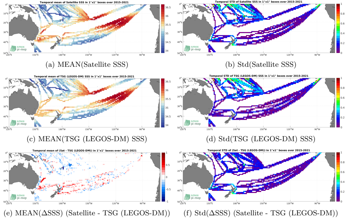
Figure 6: Temporal mean (left) and Std (right) of SSS from SMAP SSS L3 v5 - Monthly (RSS) (top), TSG (LEGOS-DM) (middle), and of \Delta SSS (Satellite - TSG (LEGOS-DM)). Only match-up pairs are used to generate these maps.
