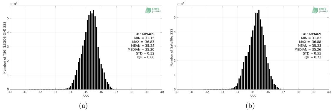
Figure 2: Histograms of SSS from TSG (LEGOS-DM) (a) and SMAP SSS L3 v5 - Monthly (RSS) (b) considering all match-up pairs per bins of 0.1 over the South Pacific Ocean Pi-MEP region and for the full satellite product period.
