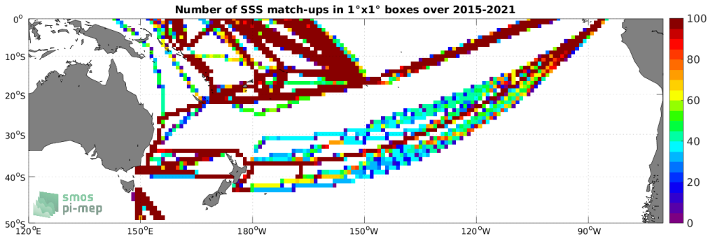
Figure 4: Number of SSS match-ups between TSG (LEGOS-DM) SSS and the SMAP SSS L3 v5 - Monthly (RSS) SSS product for the South Pacific Ocean Pi-MEP region over 1^\circ \times 1^\circ boxes and for the full satellite product period.
