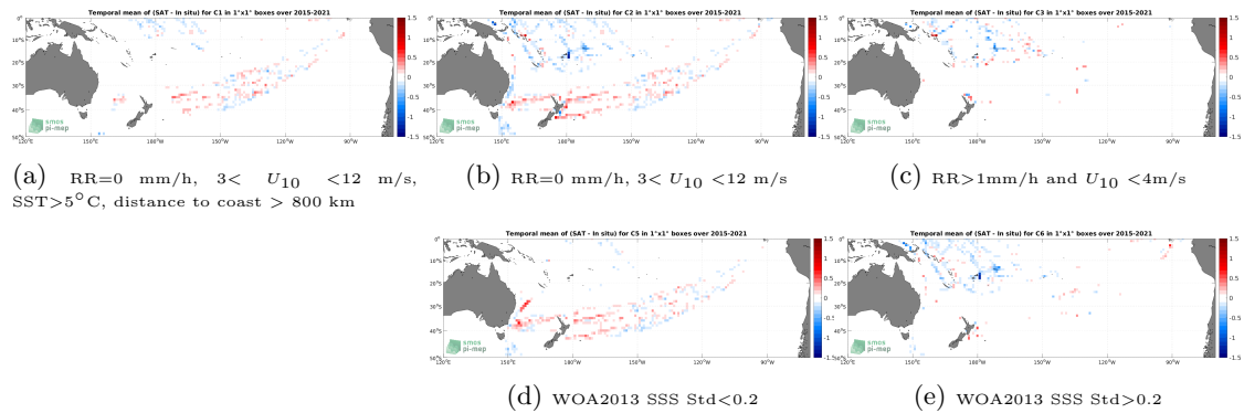
Figure 12: Temporal mean gridded over spatial boxes of size 1^\circ \times 1^\circ of \Delta\text{SSS} (SMAP SSS L3 v5 - Monthly (RSS) - TSG (LEGOS-DM)) for 5 different subdatasets corresponding to:RR=0 mm/h, 3 < U_{10} < 12 m/s, SST >5^\circ\text{C} , distance to coast > 800 km (a), RR=0 mm/h, 3 < U_{10} < 12 m/s (b), RR >1 mm/h and U_{10} < 4 m/s (c), WOA2013 SSS Std <0.2 (d), WOA2013 SSS Std >0.2 (e).
