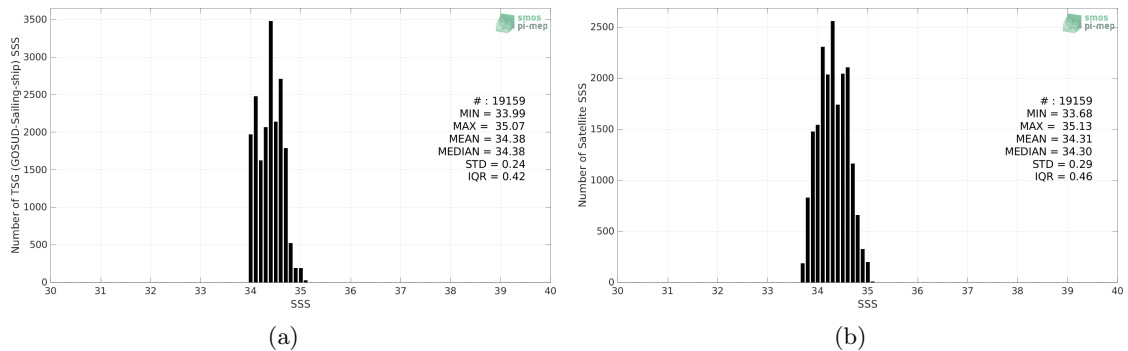
Figure 2: Histograms of SSS from TSG (GOSUD-Sailing-ship) (a) and SMAP SSS L3 v5 - Monthly (RSS) (b) considering all match-up pairs per bins of 0.1 over the South Pacific Ocean Pi-MEP region and for the full satellite product period.
