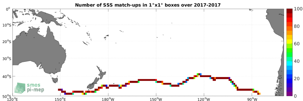
Figure 4: Number of SSS match-ups between TSG (GOSUD-Sailing-ship) SSS and the SMAP SSS L3 v5 - Monthly (RSS) SSS product for the South Pacific Ocean Pi-MEP region over 1^\circ \times 1^\circ boxes and for the full satellite product period.
