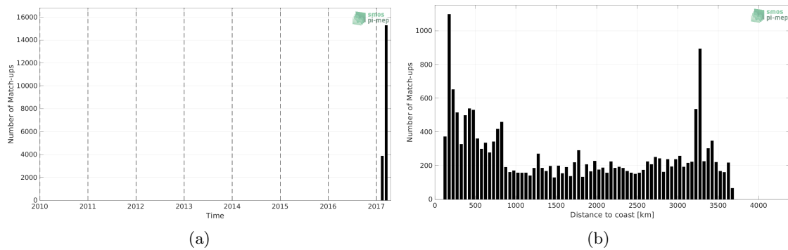
Figure 1: Number of match-ups between TSG (GOSUD-Sailing-ship) and SMAP SSS L3 v5 - Monthly (RSS) SSS as a function of time (a) and as function of the distance to coast (b) over the South Pacific Ocean Pi-MEP region and for the full satellite product period.
