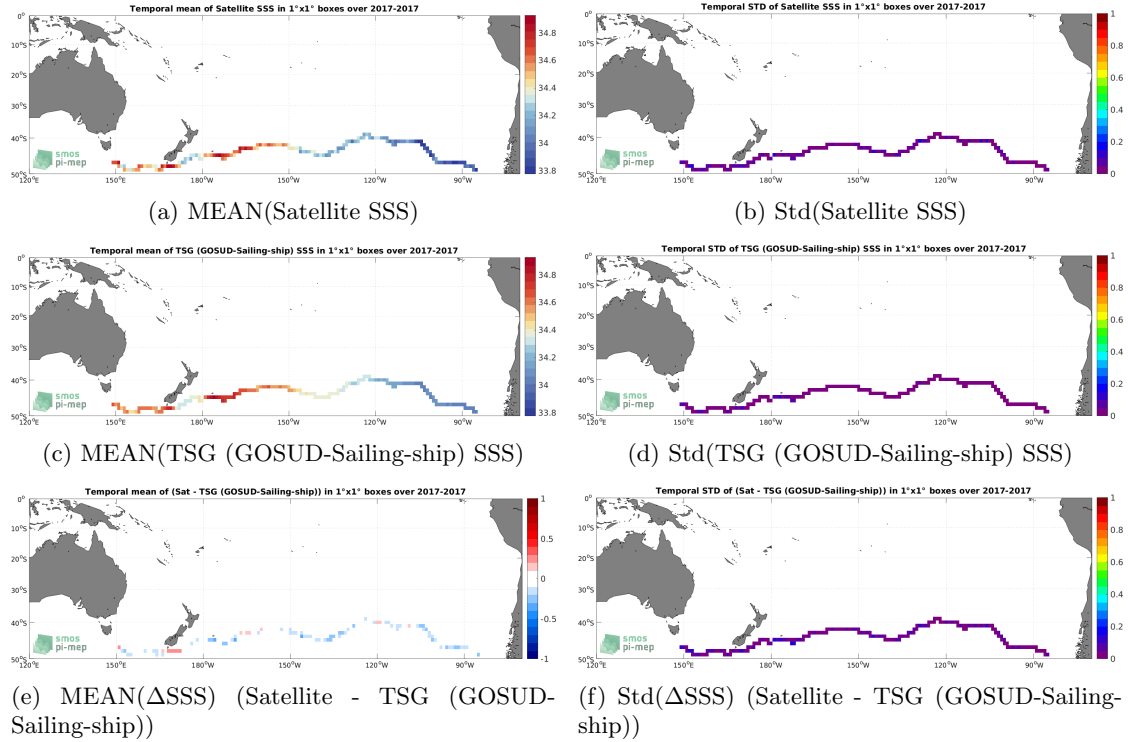
Figure 6: Temporal mean (left) and Std (right) of SSS from SMAP SSS L3 v5 - Monthly (RSS) (top), TSG (GOSUD-Sailing-ship) (middle), and of \Delta SSS (Satellite - TSG (GOSUD-Sailing-ship)). Only match-up pairs are used to generate these maps.
