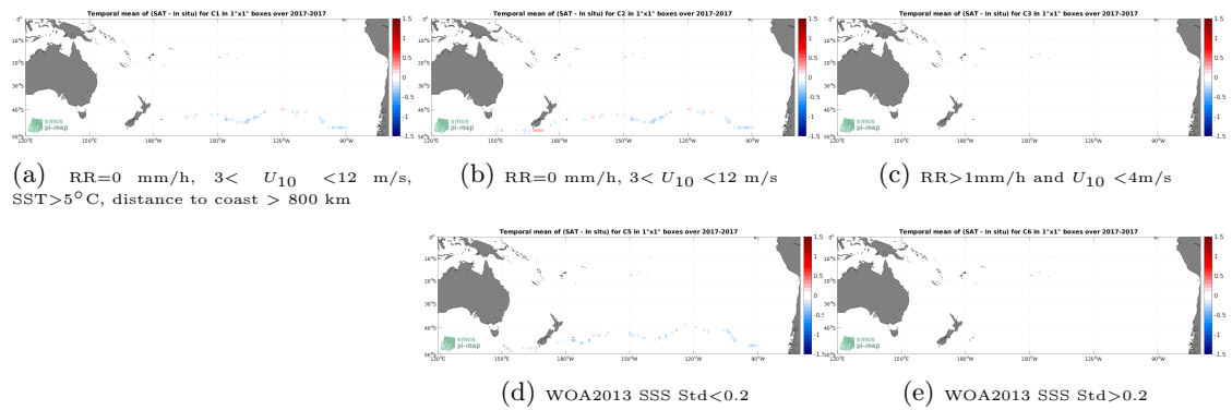
Figure 12: Temporal mean gridded over spatial boxes of size 1^\circ \times 1^\circ of \Delta SSS (SMAP SSS L3 v5 - Monthly (RSS) - TSG (GOSUD-Sailing-ship)) for 5 different subdatasets corresponding to:RR=0 mm/h, 3 < U_{10} < 12 m/s, SST>5°C, distance to coast > 800 km (a), RR=0 mm/h, 3 < U_{10} < 12 m/s (b), RR>1mm/h and U_{10} < 4 m/s (c), WOA2013 SSS Std<0.2 (d), WOA2013 SSS Std>0.2 (e).
