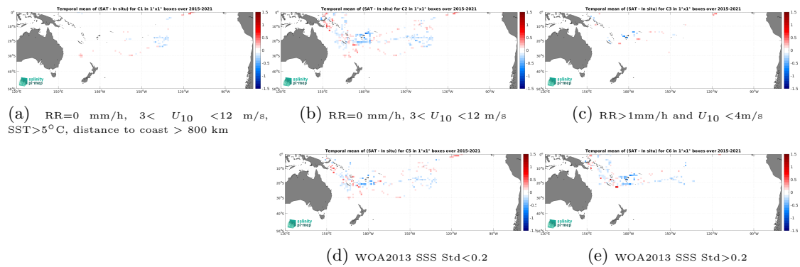
Figure 12: Temporal mean gridded over spatial boxes of size 1^\circ \times 1^\circ of \Delta\text{SSS} (SMAP SSS L3 v5 - Monthly (RSS) - TSG (GOSUD-Research-vessel)) for 5 different subdatasets corresponding to:RR=0 mm/h, 3 < U_{10} < 12 m/s, SST>5°C, distance to coast > 800 km (a), RR=0 mm/h, 3 < U_{10} < 12 m/s (b), RR>1mm/h and U_{10} < 4 m/s (c), WOA2013 SSS Std<0.2 (d), WOA2013 SSS Std>0.2 (e).
