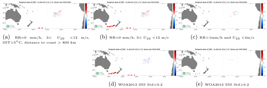
Figure 11: Temporal mean gridded over spatial boxes of size 1^\circ \times 1^\circ of \Delta SSS (SMAP SSS L3 v5 - Monthly (RSS) - Surface drifters) for 5 different subdatasets corresponding to:RR=0 mm/h, 3 < U_{10} < 12 m/s, SST > 5^\circ C , distance to coast > 800 km (a), RR=0 mm/h, 3 < U_{10} < 12 m/s (b), RR>1mm/h and U_{10} < 4 m/s (c), WOA2013 SSS Std<0.2 (d), WOA2013 SSS Std>0.2 (e).
