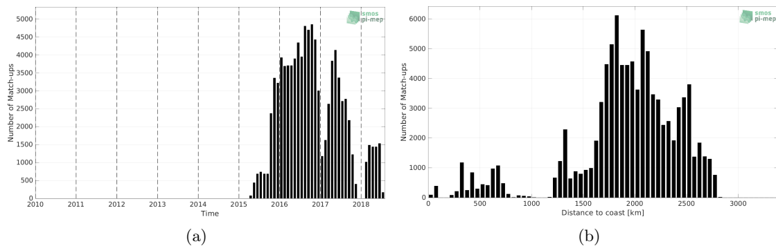
Figure 1: Number of match-ups between Surface drifters and SMAP SSS L3 v5 - Monthly (RSS) SSS as a function of time (a) and as function of the distance to coast (b) over the South Pacific Ocean Pi-MEP region and for the full satellite product period.
