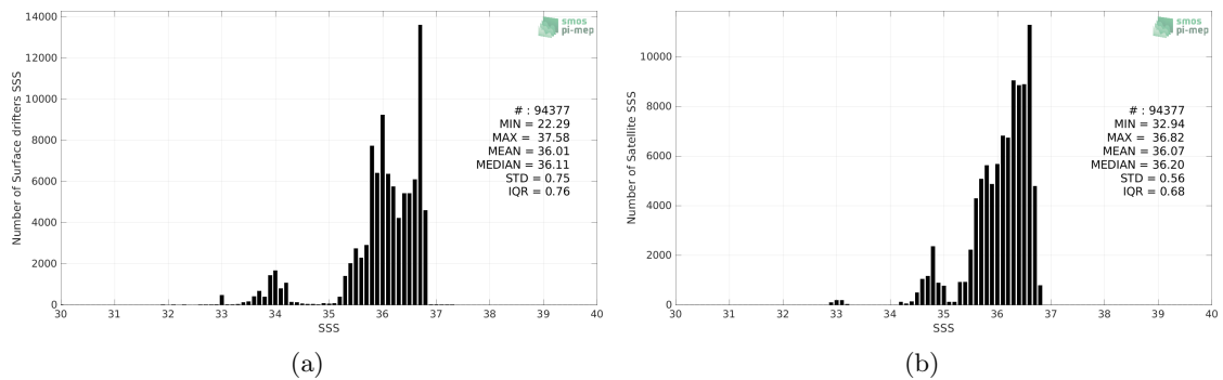
Figure 2: Histograms of SSS from Surface drifters (a) and SMAP SSS L3 v5 - Monthly (RSS) (b) considering all match-up pairs per bins of 0.1 over the South Pacific Ocean Pi-MEP region and for the full satellite product period.
