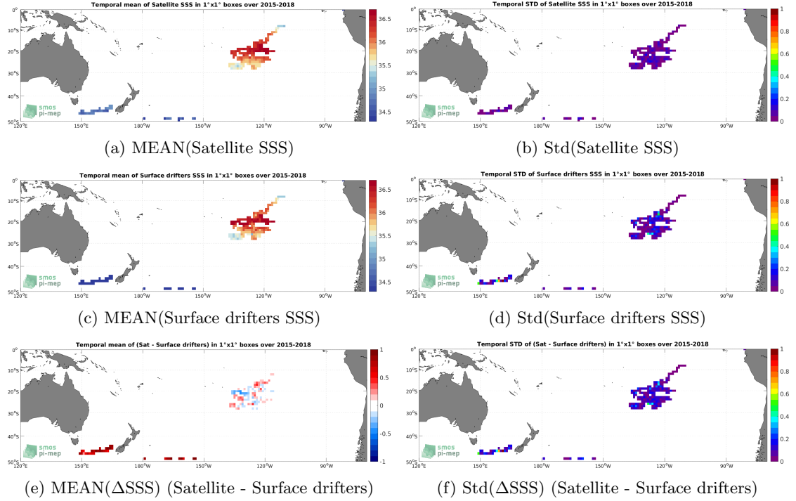
Figure 5: Temporal mean (left) and Std (right) of SSS from SMAP SSS L3 v5 - Monthly (RSS) (top), Surface drifters (middle), and of \Delta\text{SSS} (Satellite - Surface drifters). Only match-up pairs are used to generate these maps.
