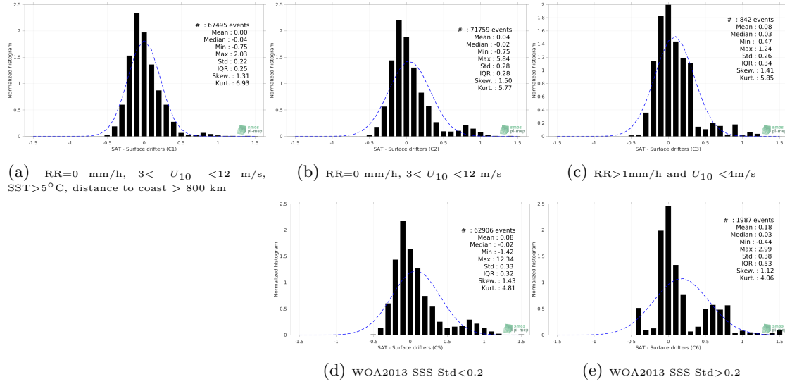
Figure 12: Normalized histogram of \Delta SSS (SMAP SSS L3 v5 - Monthly (RSS) - Surface drifters) for 5 different subdatasets corresponding to: RR=0 mm/h, 3 < U_{10} < 12 m/s, SST>5°C, distance to coast > 800 km (a), RR=0 mm/h, 3 < U_{10} < 12 m/s (b), RR>1mm/h and U_{10} < 4 m/s (c), WOA2013 SSS Std<0.2 (d), WOA2013 SSS Std>0.2 (e).
