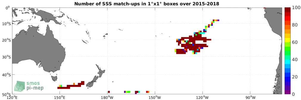
Figure 3: Number of SSS match-ups between Surface drifters SSS and the SMAP SSS L3 v5 - Monthly (RSS) SSS product for the South Pacific Ocean Pi-MEP region over 1^\circ \times 1^\circ boxes and for the full satellite product period.
