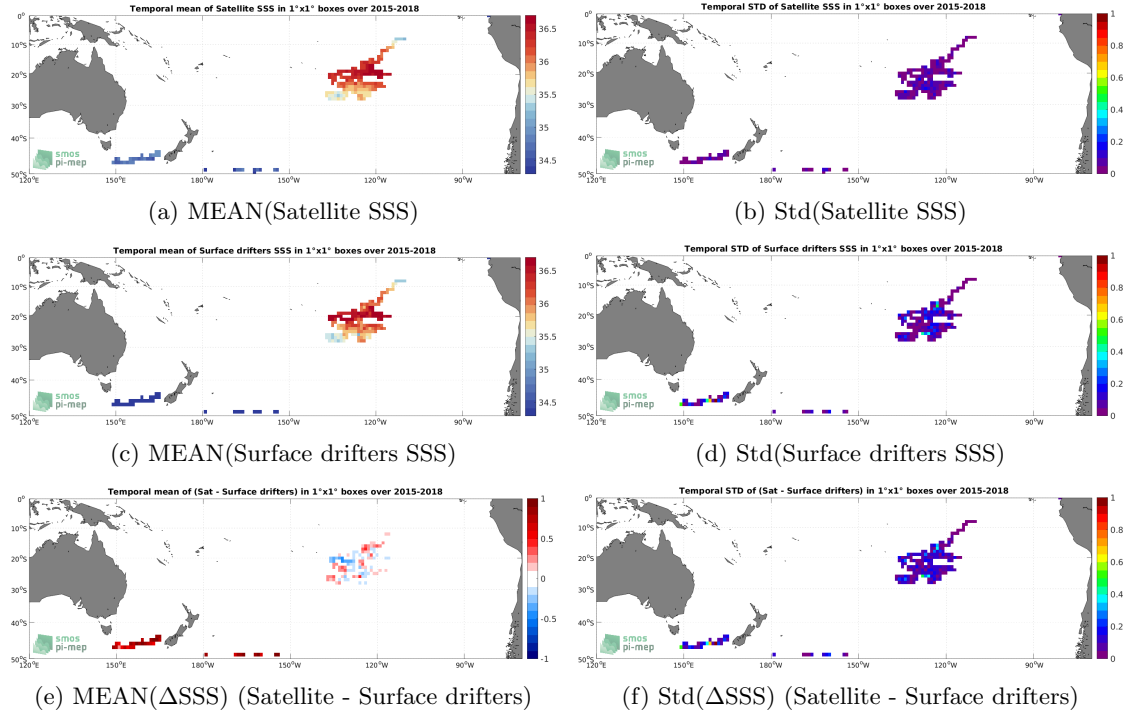
Figure 5: Temporal mean (left) and Std (right) of SSS from SMAP SSS L3 v5 - Monthly (RSS) (top), Surface drifters (middle), and of \Delta SSS (Satellite - Surface drifters). Only match-up pairs are used to generate these maps.
