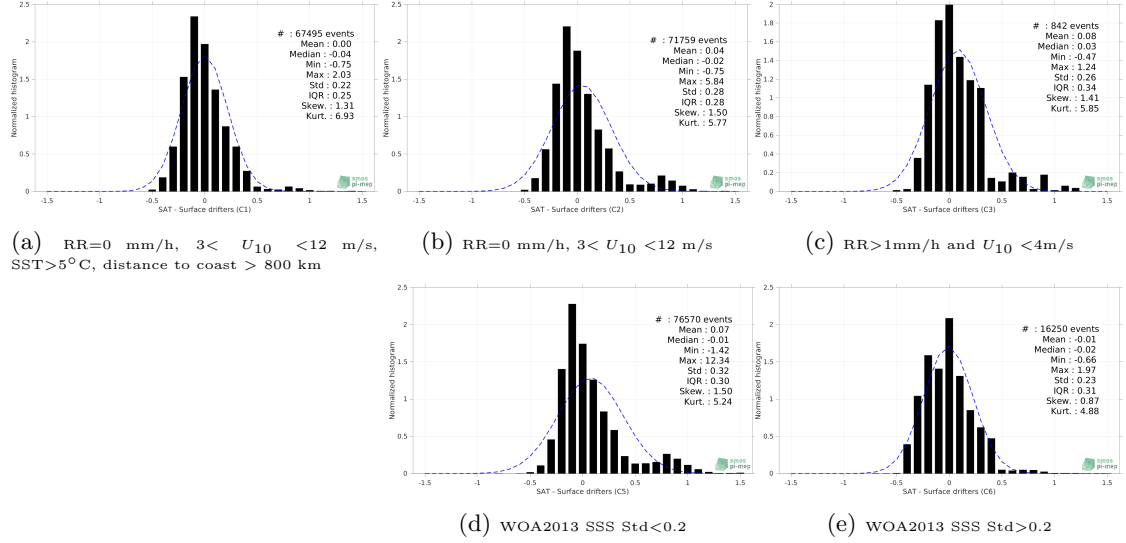
Figure 12: Normalized histogram of \Delta SSS (SMAP SSS L3 v5 - Monthly (RSS) - Surface drifters) for 5 different subdatasets corresponding to: RR=0 mm/h, 3 < U_{10} < 12 m/s, SST>5°C, distance to coast > 800 km (a), RR=0 mm/h, 3 < U_{10} < 12 m/s (b), RR>1mm/h and U_{10} < 4 m/s (c), WOA2013 SSS Std<0.2 (d), WOA2013 SSS Std>0.2 (e).
