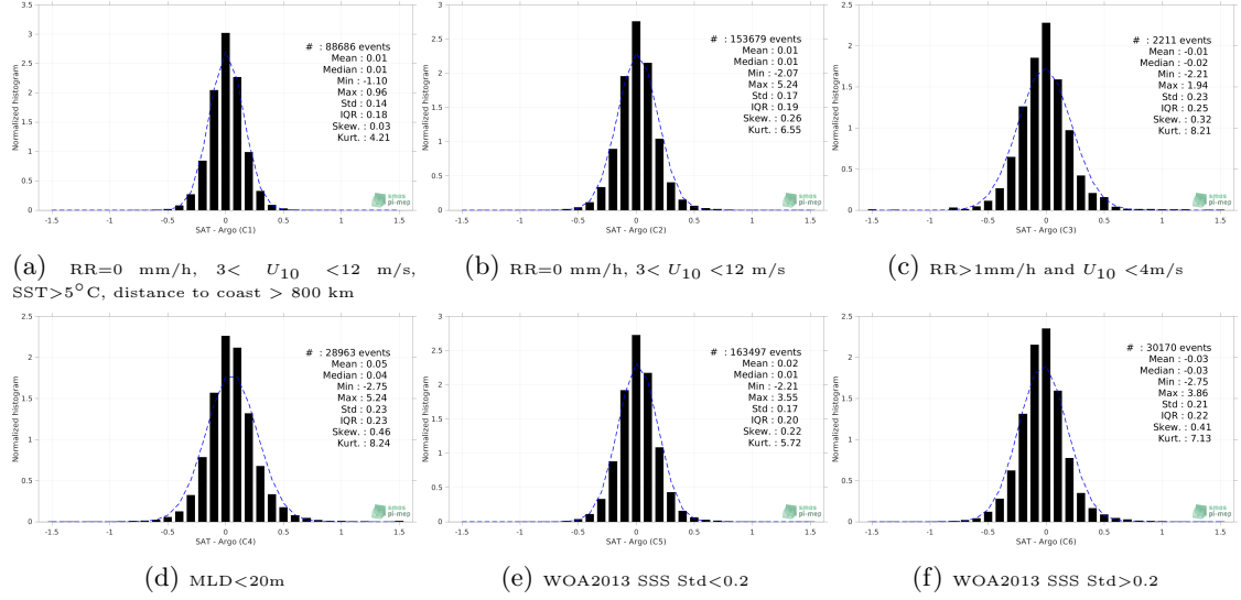
Figure 13: Normalized histogram of \Delta SSS (SMAP SSS L3 v5 - Monthly (RSS) - Argo) for 6 different subdatasets corresponding to: RR=0 mm/h, 3 < U_{10} < 12 m/s, SST>5°C, distance to coast > 800 km (a), RR=0 mm/h, 3 < U_{10} < 12 m/s (b), RR>1mm/h and U_{10} < 4 m/s (c), MLD<20m (d), WOA2013 SSS Std<0.2 (e), WOA2013 SSS Std>0.2 (f).
