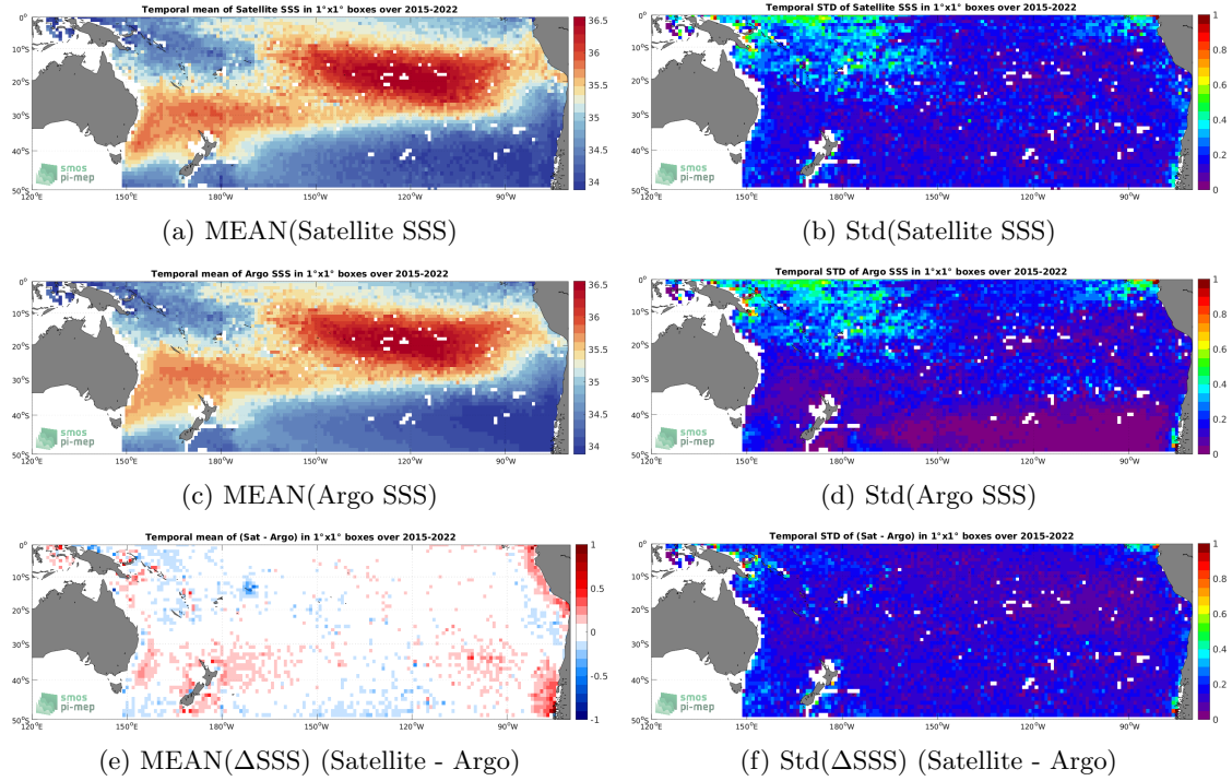
Figure 6: Temporal mean (left) and Std (right) of SSS from SMAP SSS L3 v5 - Monthly (RSS) (top), Argo (middle), and of \Delta SSS (Satellite - Argo). Only match-up pairs are used to generate these maps.
