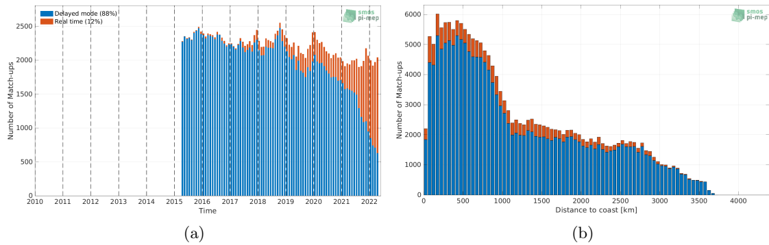
Figure 1: Number of match-ups between Argo and SMAP SSS L3 v5 - Monthly (RSS) SSS as a function of time (a) and as function of the distance to coast (b) over the South Pacific Ocean Pi-MEP region and for the full satellite product period.
