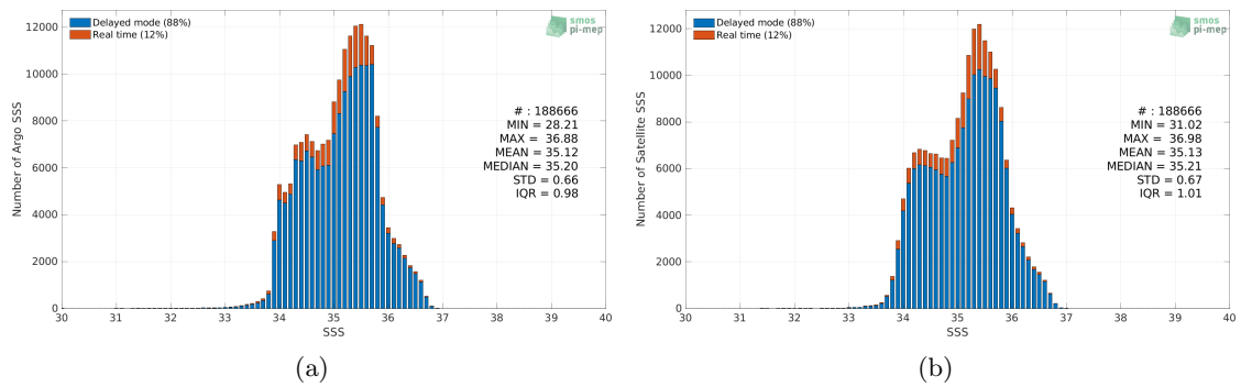
Figure 2: Histograms of SSS from Argo (a) and SMAP SSS L3 v5 - Monthly (RSS) (b) considering all match-up pairs per bins of 0.1 over the South Pacific Ocean Pi-MEP region and for the full satellite product period.
