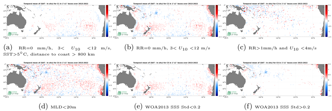
Figure 12: Temporal mean gridded over spatial boxes of size 1^\circ \times 1^\circ of \Delta SSS (SMAP SSS L3 v5 - Monthly (RSS) - Argo) for 6 different subdatasets corresponding to:RR=0 mm/h, 3 < U_{10} < 12 m/s, SST >5^\circ C, distance to coast > 800 km (a), RR=0 mm/h, 3 < U_{10} < 12 m/s (b), RR >1 mm/h and U_{10} < 4 m/s (c),MLD <20 m (d),WOA2013 SSS Std <0.2 (e),WOA2013 SSS Std >0.2 (f).
