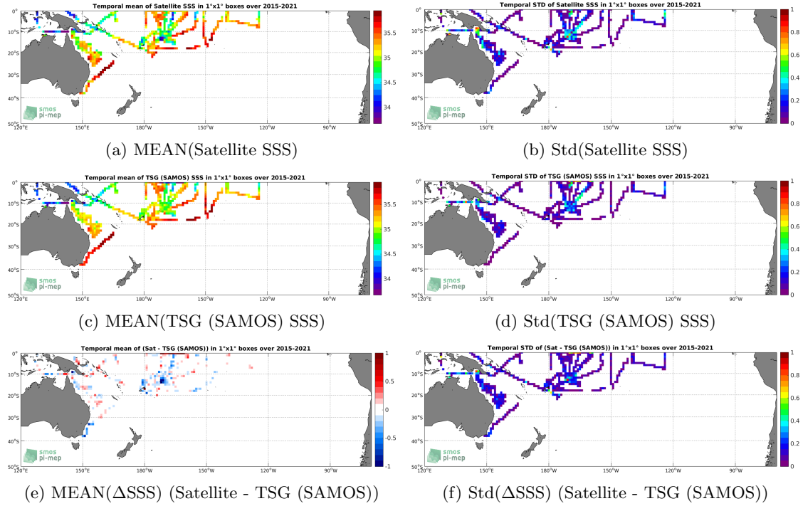
Figure 6: Temporal mean (left) and Std (right) of SSS from SMAP SSS L3 v4 - 8-Day running (RSS) (top), TSG (SAMOS) (middle), and of \Delta SSS (Satellite - TSG (SAMOS)). Only match-up pairs are used to generate these maps.
