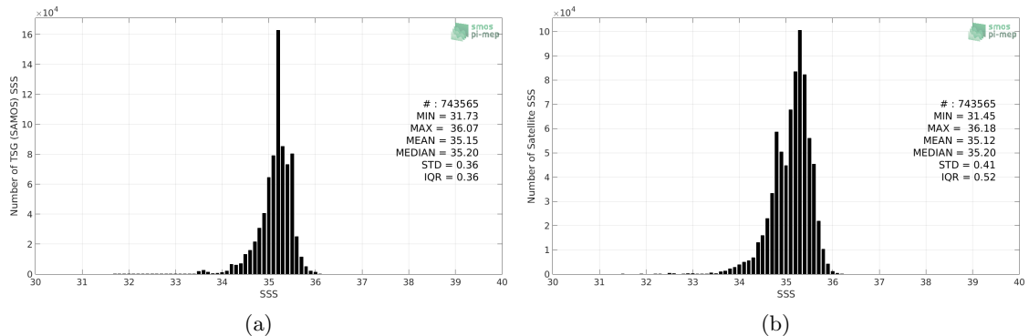
Figure 2: Histograms of SSS from TSG (SAMOS) (a) and SMAP SSS L3 v4 - 8-Day running (RSS) (b) considering all match-up pairs per bins of 0.1 over the South Pacific Ocean Pi-MEP region and for the full satellite product period.
