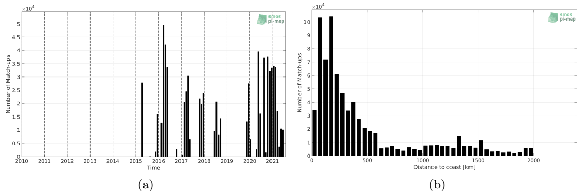
Figure 1: Number of match-ups between TSG (SAMOS) and SMAP SSS L3 v4 - 8-Day running (RSS) SSS as a function of time (a) and as function of the distance to coast (b) over the South Pacific Ocean Pi-MEP region and for the full satellite product period.
