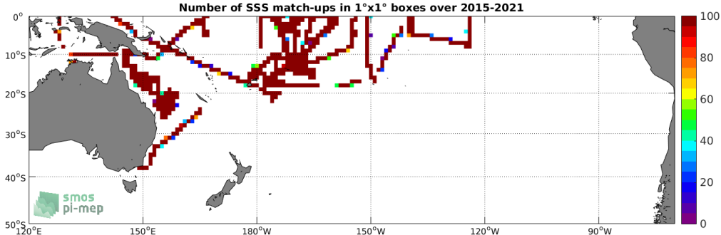
Figure 4: Number of SSS match-ups between TSG (SAMOS) SSS and the SMAP SSS L3 v4 - 8-Day running (RSS) SSS product for the South Pacific Ocean Pi-MEP region over 1^\circ \times 1^\circ boxes and for the full satellite product period.
