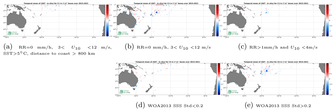
Figure 12: Temporal mean gridded over spatial boxes of size 1^\circ \times 1^\circ of \Delta SSS (SMAP SSS L3 v4 - 8-Day running (RSS) - TSG (SAMOS)) for 5 different subdatasets corresponding to:RR=0 mm/h, 3 < U_{10} < 12 m/s, SST >5^\circ C, distance to coast > 800 km (a), RR=0 mm/h, 3 < U_{10} < 12 m/s (b), RR >1 mm/h and U_{10} < 4 m/s (c), WOA2013 SSS Std <0.2 (d), WOA2013 SSS Std >0.2 (e).
