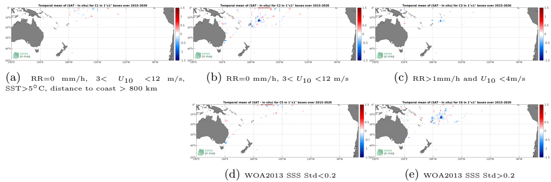
Figure 12: Temporal mean gridded over spatial boxes of size 1^\circ \times 1^\circ of \Delta\text{SSS} (SMAP SSS L3 v4 - 8-Day running (RSS) - TSG (SAMOS)) for 5 different subdatasets corresponding to:RR=0 mm/h, 3 < U_{10} < 12 m/s, SST >5^\circ\text{C} , distance to coast > 800 km (a), RR=0 mm/h, 3 < U_{10} < 12 m/s (b), RR >1 mm/h and U_{10} < 4 m/s (c), WOA2013 SSS Std <0.2 (d), WOA2013 SSS Std >0.2 (e).
