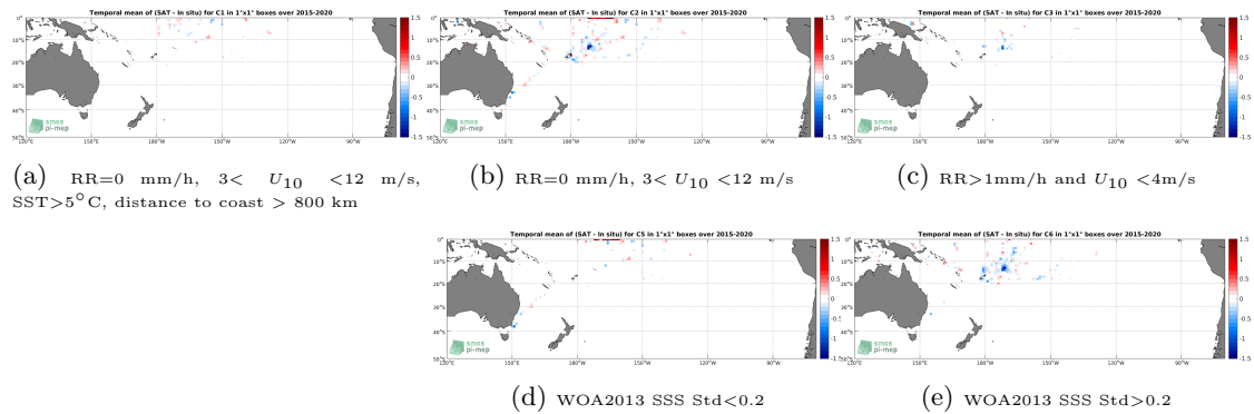
Figure 12: Temporal mean gridded over spatial boxes of size 1^\circ \times 1^\circ of \Delta SSS (SMAP-L3-RSS-V4-8DAY-RUNNING - TSG-SAMOS) for 5 different subdatasets corresponding to:RR=0 mm/h, 3 < U_{10} < 12 m/s, SST >5^\circ\text{C} , distance to coast > 800 km (a), RR=0 mm/h, 3 < U_{10} < 12 m/s (b), RR >1 mm/h and U_{10} < 4 m/s (c), WOA2013 SSS Std <0.2 (d), WOA2013 SSS Std >0.2 (e).
