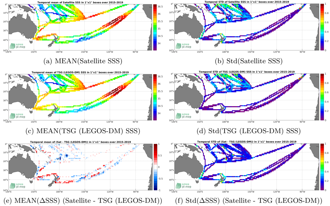
Figure 6: Temporal mean (left) and Std (right) of SSS from SMAP SSS L3 v4 - 8-Day running (RSS) (top), TSG (LEGOS-DM) (middle), and of \Delta SSS (Satellite - TSG (LEGOS-DM)). Only match-up pairs are used to generate these maps.
