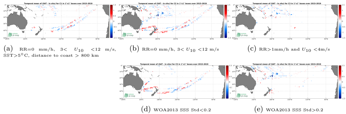
Figure 12: Temporal mean gridded over spatial boxes of size 1^\circ \times 1^\circ of \Delta\text{SSS} (SMAP SSS L3 v4 - 8-Day running (RSS) - TSG (LEGOS-DM)) for 5 different subdatasets corresponding to: \text{RR}=0 mm/h, 3 < U_{10} < 12 m/s, \text{SST} > 5^\circ\text{C} , distance to coast > 800 km (a), \text{RR}=0 mm/h, 3 < U_{10} < 12 m/s (b), \text{RR} > 1 mm/h and U_{10} < 4 m/s (c), WOA2013 SSS Std < 0.2 (d), WOA2013 SSS Std > 0.2 (e).
