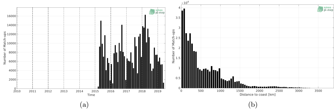
Figure 1: Number of match-ups between TSG (LEGOS-DM) and SMAP SSS L3 v4 - 8-Day running (RSS) SSS as a function of time (a) and as function of the distance to coast (b) over the South Pacific Ocean Pi-MEP region and for the full satellite product period.
