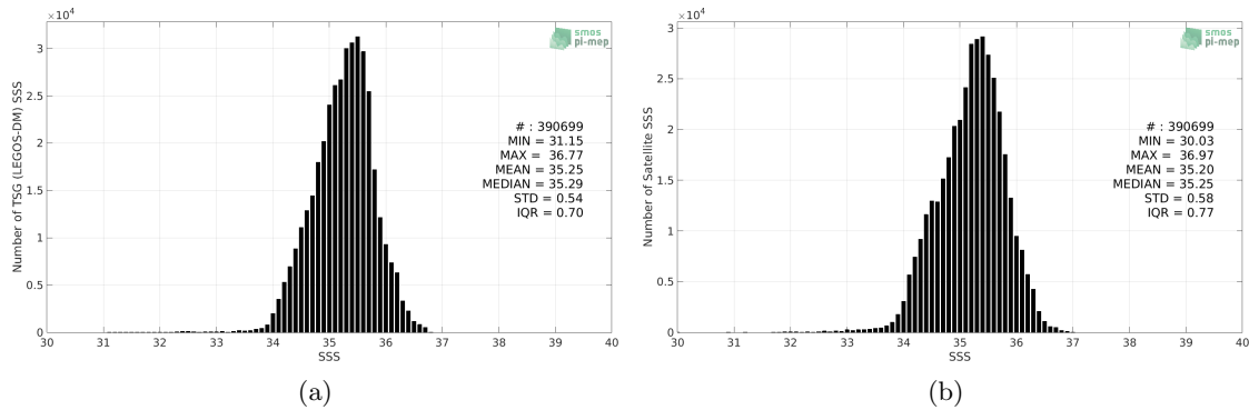
Figure 2: Histograms of SSS from TSG (LEGOS-DM) (a) and SMAP SSS L3 v4 - 8-Day running (RSS) (b) considering all match-up pairs per bins of 0.1 over the South Pacific Ocean Pi-MEP region and for the full satellite product period.
