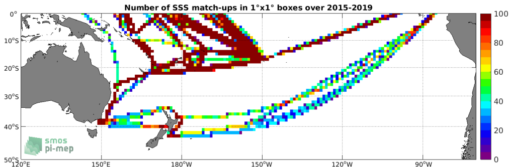
Figure 4: Number of SSS match-ups between TSG (LEGOS-DM) SSS and the SMAP SSS L3 v4 - 8-Day running (RSS) SSS product for the South Pacific Ocean Pi-MEP region over 1^\circ \times 1^\circ boxes and for the full satellite product period.
