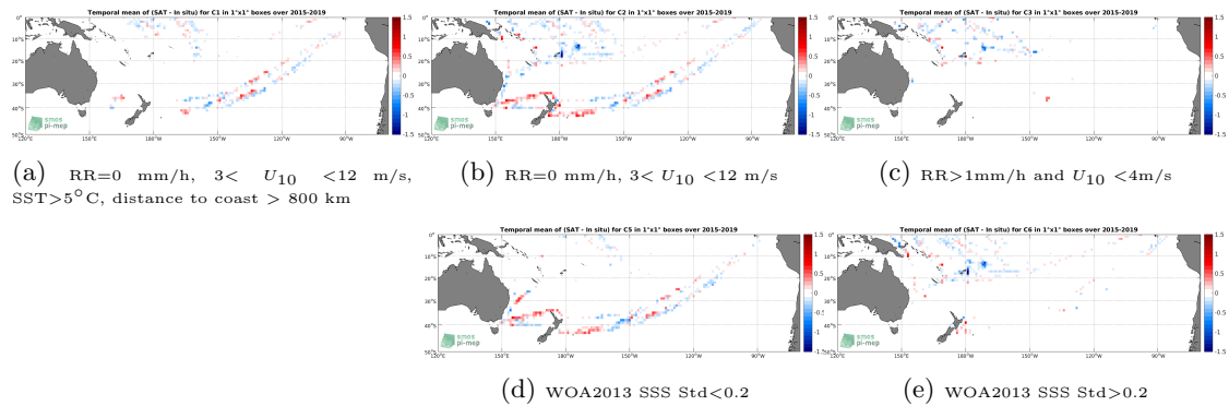
Figure 12: Temporal mean gridded over spatial boxes of size 1^\circ \times 1^\circ of \Delta SSS (SMAP-L3-RSS-V4-8DAY-RUNNING - TSG-LEGOS-DM) for 5 different subdatasets corresponding to: RR=0 mm/h, 3 < U_{10} < 12 m/s, SST > 5^\circ C , distance to coast > 800 km (a), RR=0 mm/h, 3 < U_{10} < 12 m/s (b), RR > 1 mm/h and U_{10} < 4 m/s (c), WOA2013 SSS Std < 0.2 (d), WOA2013 SSS Std > 0.2 (e).
