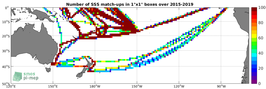
Figure 4: Number of SSS match-ups between TSG-LEGOS-DM SSS and the SMAP-L3-RSS-V4-8DAY-RUNNING SSS product for the South Pacific Ocean Pi-MEP region over 1°x1° boxes and for the full satellite product period.
