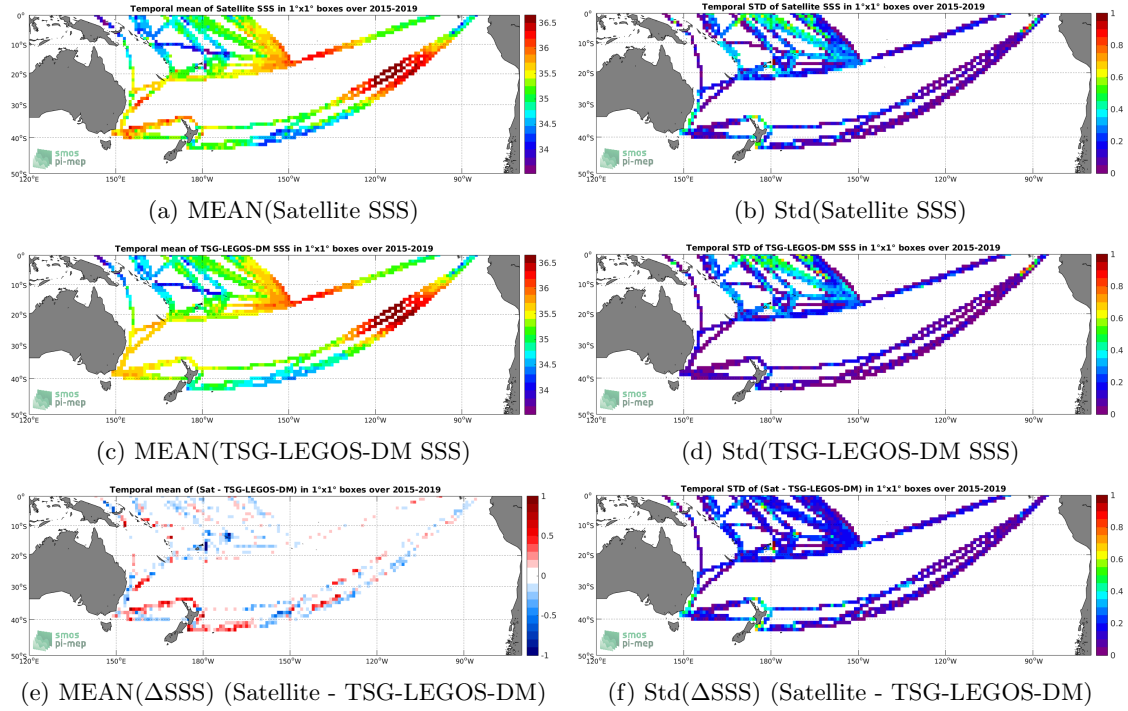
Figure 6: Temporal mean (left) and Std (right) of SSS from SMAP-L3-RSS-V4-8DAY-RUNNING (top), TSG-LEGOS-DM (middle), and of \Delta SSS (Satellite - TSG-LEGOS-DM). Only match-up pairs are used to generate these maps.
