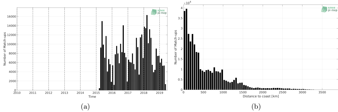
Figure 1: Number of match-ups between TSG-LEGOS-DM and SMAP-L3-RSS-V4-8DAY-RUNNING SSS as a function of time (a) and as function of the distance to coast (b) over the South Pacific Ocean Pi-MEP region and for the full satellite product period.
