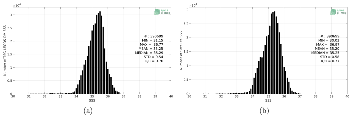
Figure 2: Histograms of SSS from TSG-LEGOS-DM (a) and SMAP-L3-RSS-V4-8DAY-RUNNING (b) considering all match-up pairs per bins of 0.1 over the South Pacific Ocean Pi-MEP region and for the full satellite product period.
