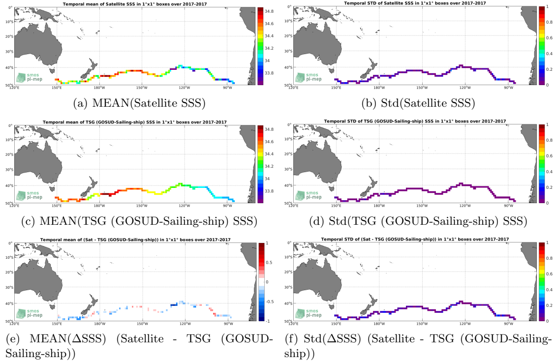
Figure 6: Temporal mean (left) and Std (right) of SSS from SMAP SSS L3 v4 - 8-Day running (RSS) (top), TSG (GOSUD-Sailing-ship) (middle), and of \Delta SSS (Satellite - TSG (GOSUD-Sailing-ship)). Only match-up pairs are used to generate these maps.
