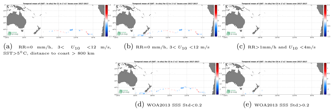
Figure 12: Temporal mean gridded over spatial boxes of size 1^\circ \times 1^\circ of \Delta\text{SSS} (SMAP SSS L3 v4 - 8-Day running (RSS) - TSG (GOSUD-Sailing-ship)) for 5 different subdatasets corresponding to: RR=0 mm/h, 3 < U_{10} < 12 m/s, SST > 5°C, distance to coast > 800 km (a), RR=0 mm/h, 3 < U_{10} < 12 m/s (b), RR > 1mm/h and U_{10} < 4 m/s (c), WOA2013 SSS Std < 0.2 (d), WOA2013 SSS Std > 0.2 (e).
