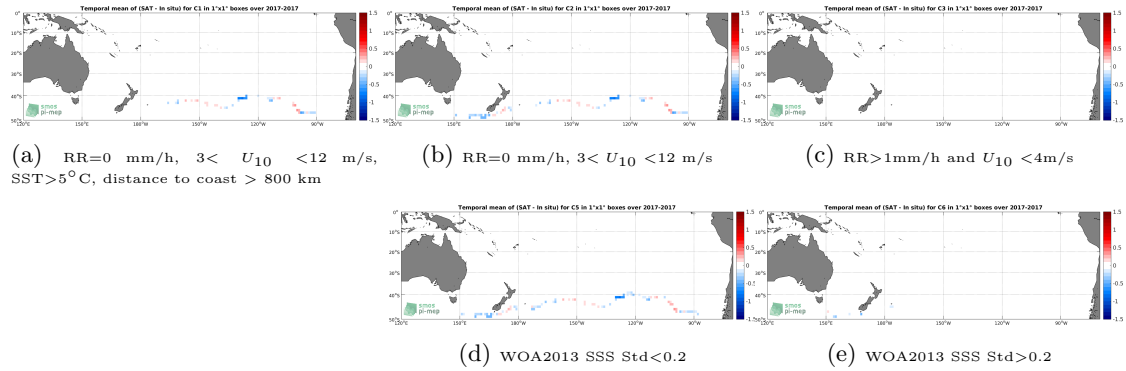
Figure 12: Temporal mean gridded over spatial boxes of size 1^{\circ}\times 1^{\circ} of \Delta SSS (SMAP-L3-RSS-V4-8DAY-RUNNING - TSG-GOSUD-Sailing-ship) for 5 different subdatasets corresponding to:RR=0 mm/h, 3 < U_{10} < 12 m/s, SST >5^{\circ}\text{C} , distance to coast > 800 km (a), RR=0 mm/h, 3 < U_{10} < 12 m/s (b), RR >1 mm/h and U_{10} < 4 m/s (c), WOA2013 SSS Std <0.2 (d), WOA2013 SSS Std >0.2 (e).
