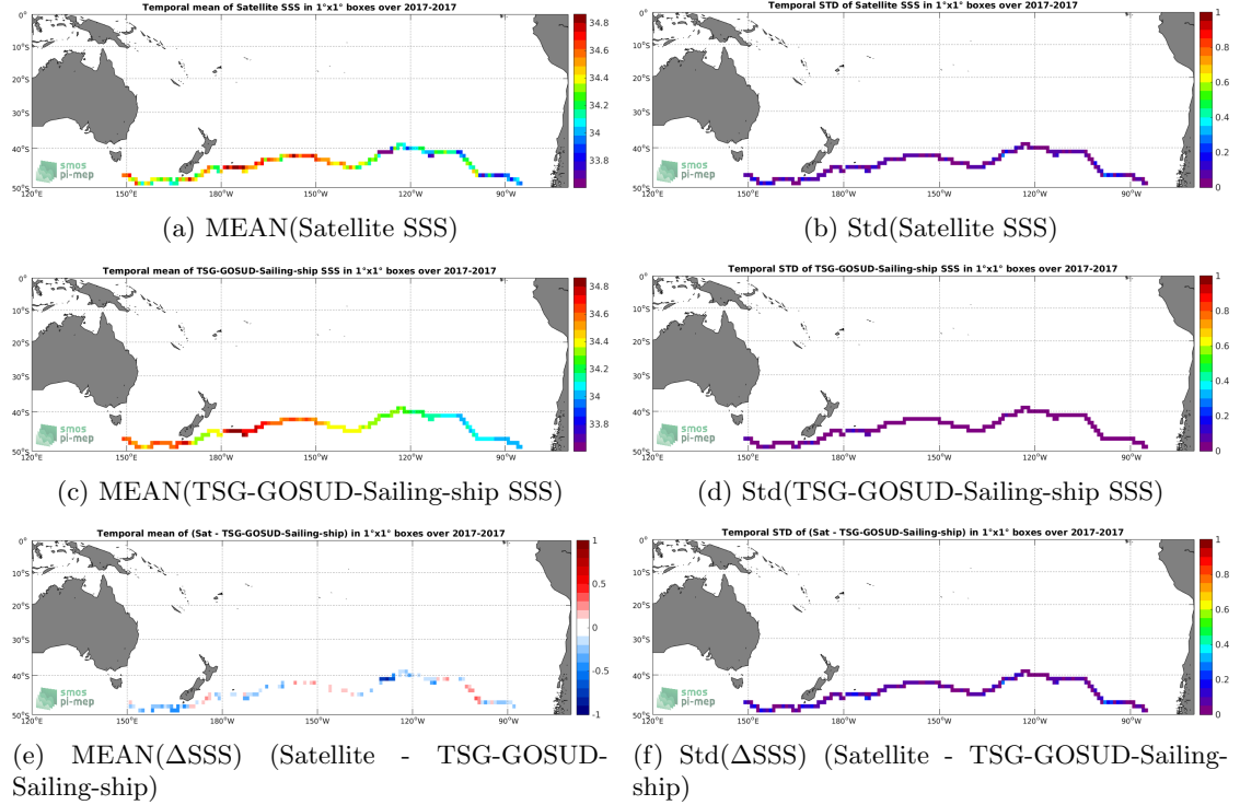
Figure 6: Temporal mean (left) and Std (right) of SSS from SMAP-L3-RSS-V4-8DAY-RUNNING (top), TSG-GOSUD-Sailing-ship (middle), and of \Delta SSS (Satellite - TSG-GOSUD-Sailing-ship). Only match-up pairs are used to generate these maps.
