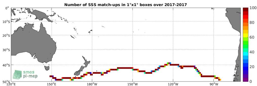
Figure 4: Number of SSS match-ups between TSG-GOSUD-Sailing-ship SSS and the SMAP-L3-RSS-V4-8DAY-RUNNING SSS product for the South Pacific Ocean Pi-MEP region over 1°x1° boxes and for the full satellite product period.
