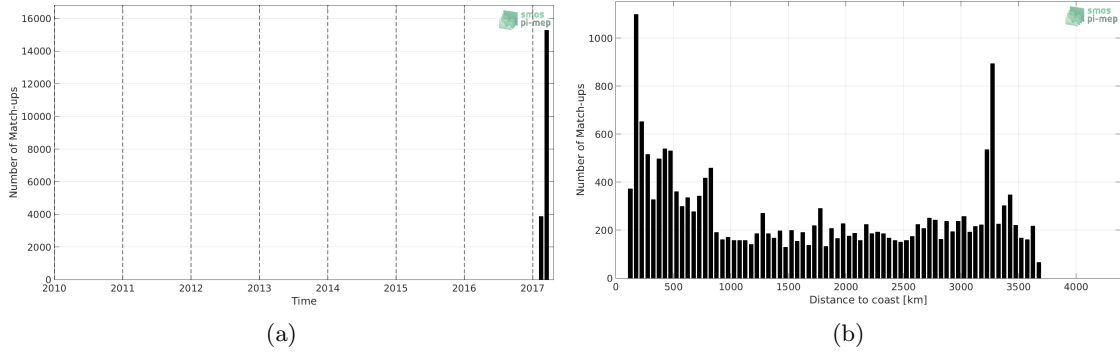
Figure 1: Number of match-ups between TSG-GOSUD-Sailing-ship and SMAP-L3-RSS-V4-8DAY-RUNNING SSS as a function of time (a) and as function of the distance to coast (b) over the South Pacific Ocean Pi-MEP region and for the full satellite product period.
