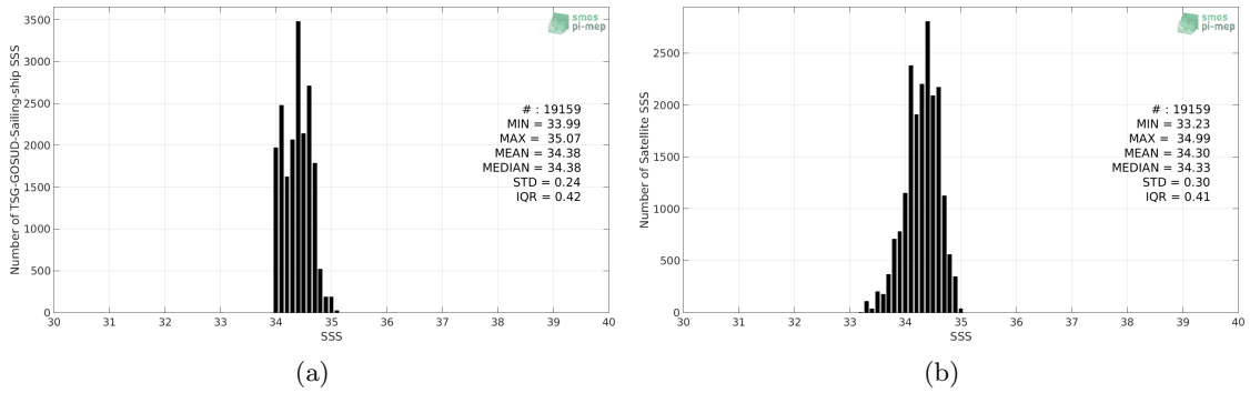
Figure 2: Histograms of SSS from TSG-GOSUD-Sailing-ship (a) and SMAP-L3-RSS-V4-8DAY-RUNNING (b) considering all match-up pairs per bins of 0.1 over the South Pacific Ocean Pi-MEP region and for the full satellite product period.
