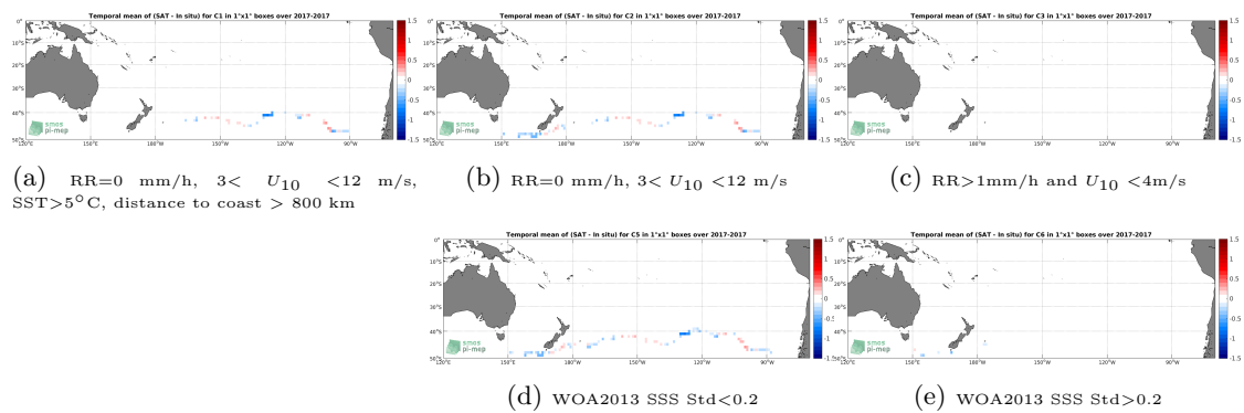
Figure 12: Temporal mean gridded over spatial boxes of size 1^\circ \times 1^\circ of \Delta SSS (SMAP-L3-RSS-V4-8DAY-RUNNING - TSG-GOSUD-Sailing-ship) for 5 different subdatasets corresponding to: RR=0 mm/h, 3 < U_{10} < 12 m/s, SST > 5°C, distance to coast > 800 km (a), RR=0 mm/h, 3 < U_{10} < 12 m/s (b), RR > 1mm/h and U_{10} < 4 m/s (c), WOA2013 SSS Std < 0.2 (d), WOA2013 SSS Std > 0.2 (e).
