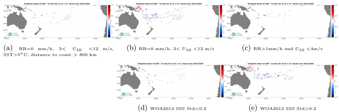
Figure 12: Temporal mean gridded over spatial boxes of size 1^\circ \times 1^\circ of \Delta SSS (SMAP SSS L3 v4 - 8-Day running (RSS) - TSG (GOSUD-Research-vessel)) for 5 different subdatasets corresponding to:RR=0 mm/h, 3 < U_{10} < 12 m/s, SST >5^\circ\text{C} , distance to coast > 800 km (a), RR=0 mm/h, 3 < U_{10} < 12 m/s (b), RR >1 mm/h and U_{10} < 4 m/s (c), WOA2013 SSS Std <0.2 (d), WOA2013 SSS Std >0.2 (e).
