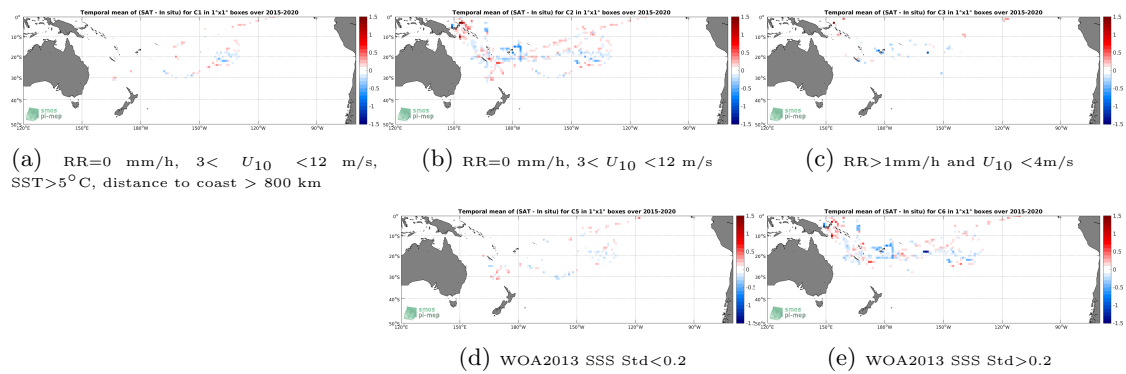
Figure 12: Temporal mean gridded over spatial boxes of size 1^\circ \times 1^\circ of \Delta\text{SSS} (SMAP SSS L3 v4 - 8-Day running (RSS) - TSG (GOSUD-Research-vessel)) for 5 different subdatasets corresponding to: RR=0 mm/h, 3 < U_{10} < 12 m/s, SST > 5°C, distance to coast > 800 km (a), RR=0 mm/h, 3 < U_{10} < 12 m/s (b), RR > 1mm/h and U_{10} < 4 m/s (c), WOA2013 SSS Std < 0.2 (d), WOA2013 SSS Std > 0.2 (e).
