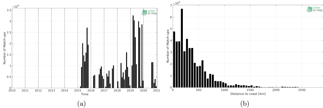
Figure 1: Number of match-ups between TSG (GOSUD-Research-vessel) and SMAP SSS L3 v4 - 8-Day running (RSS) SSS as a function of time (a) and as function of the distance to coast (b) over the South Pacific Ocean Pi-MEP region and for the full satellite product period.
