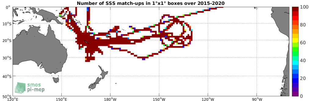
Figure 4: Number of SSS match-ups between TSG (GOSUD-Research-vessel) SSS and the SMAP SSS L3 v4 - 8-Day running (RSS) SSS product for the South Pacific Ocean Pi-MEP region over 1^\circ \times 1^\circ boxes and for the full satellite product period.
