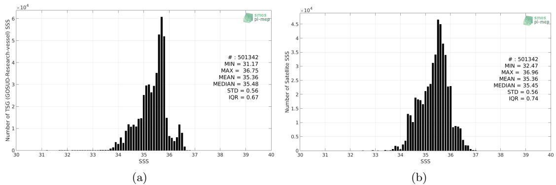
Figure 2: Histograms of SSS from TSG (GOSUD-Research-vessel) (a) and SMAP SSS L3 v4 - 8-Day running (RSS) (b) considering all match-up pairs per bins of 0.1 over the South Pacific Ocean Pi-MEP region and for the full satellite product period.
