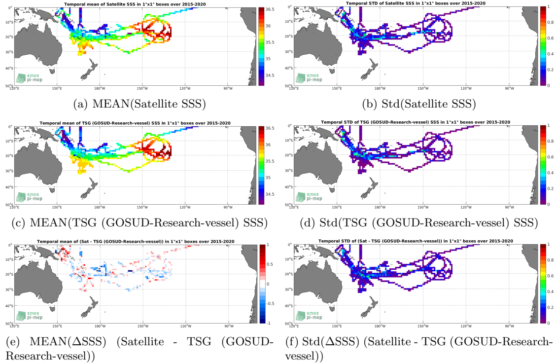
Figure 6: Temporal mean (left) and Std (right) of SSS from SMAP SSS L3 v4 - 8-Day running (RSS) (top), TSG (GOSUD-Research-vessel) (middle), and of \Delta SSS (Satellite - TSG (GOSUD-Research-vessel)). Only match-up pairs are used to generate these maps.
