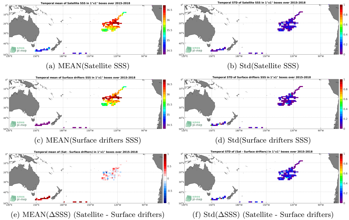
Figure 5: Temporal mean (left) and Std (right) of SSS from SMAP SSS L3 v4 - 8-Day running (RSS) (top), Surface drifters (middle), and of \Delta SSS (Satellite - Surface drifters). Only match-up pairs are used to generate these maps.
