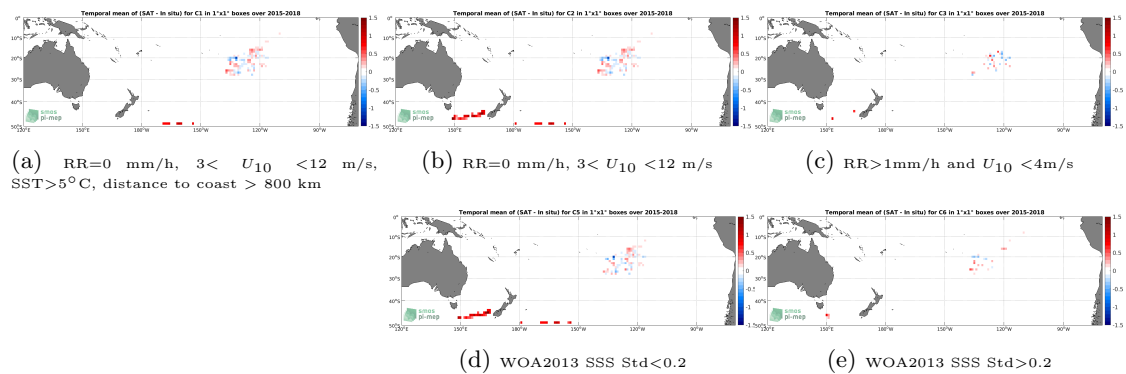
Figure 11: Temporal mean gridded over spatial boxes of size 1^\circ \times 1^\circ of \Delta SSS (SMAP SSS L3 v4 - 8-Day running (RSS) - Surface drifters) for 5 different subdatasets corresponding to:RR=0 mm/h, 3 < U_{10} < 12 m/s, SST >5^\circ C, distance to coast > 800 km (a), RR=0 mm/h, 3 < U_{10} < 12 m/s (b), RR >1 mm/h and U_{10} < 4 m/s (c), WOA2013 SSS Std <0.2 (d), WOA2013 SSS Std >0.2 (e).
