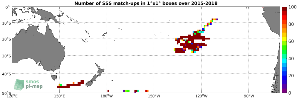
Figure 3: Number of SSS match-ups between Surface drifters SSS and the SMAP SSS L3 v4 - 8-Day running (RSS) SSS product for the South Pacific Ocean Pi-MEP region over 1^\circ \times 1^\circ boxes and for the full satellite product period.
