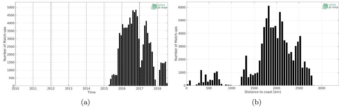
Figure 1: Number of match-ups between Surface drifters and SMAP SSS L3 v4 - 8-Day running (RSS) SSS as a function of time (a) and as function of the distance to coast (b) over the South Pacific Ocean Pi-MEP region and for the full satellite product period.
