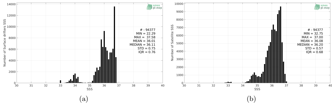
Figure 2: Histograms of SSS from Surface drifters (a) and SMAP SSS L3 v4 - 8-Day running (RSS) (b) considering all match-up pairs per bins of 0.1 over the South Pacific Ocean Pi-MEP region and for the full satellite product period.
