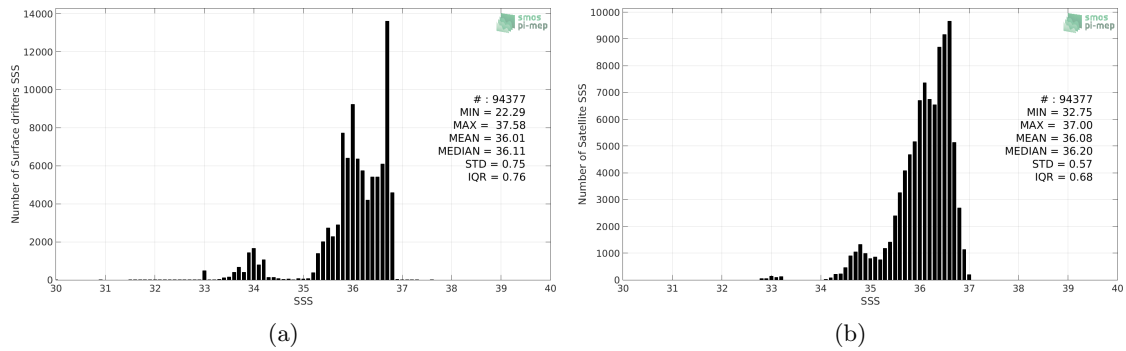
Figure 2: Histograms of SSS from Surface drifters (a) and SMAP-L3-RSS-V4-8DAY-RUNNING (b) considering all match-up pairs per bins of 0.1 over the South Pacific Ocean Pi-MEP region and for the full satellite product period.
