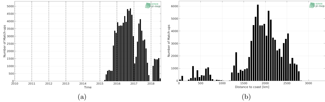
Figure 1: Number of match-ups between Surface drifters and SMAP-L3-RSS-V4-8DAY-RUNNING SSS as a function of time (a) and as function of the distance to coast (b) over the South Pacific Ocean Pi-MEP region and for the full satellite product period.
