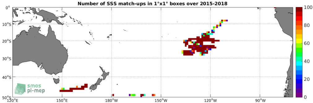
Figure 3: Number of SSS match-ups between Surface drifters SSS and the SMAP-L3-RSS-V4-8DAY-RUNNING SSS product for the South Pacific Ocean Pi-MEP region over 1^\circ \times 1^\circ boxes and for the full satellite product period.
