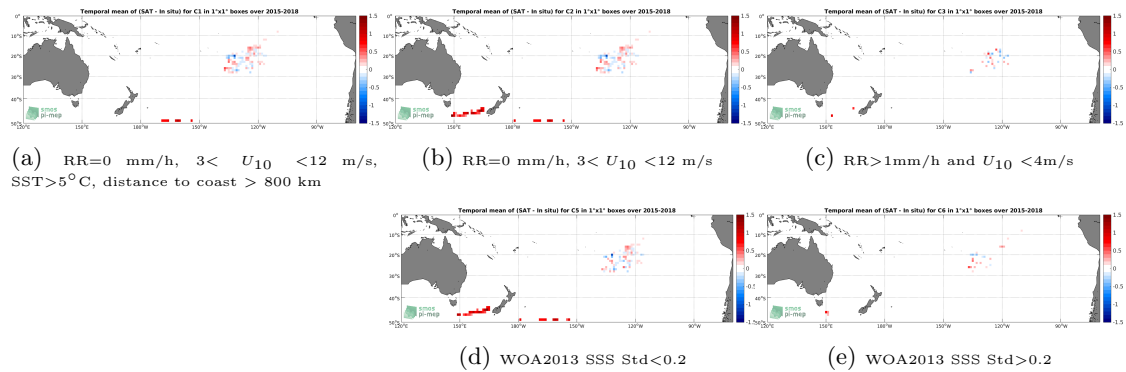
Figure 11: Temporal mean gridded over spatial boxes of size 1^\circ \times 1^\circ of \Delta SSS (SMAP-L3-RSS-V4-8DAY-RUNNING - Surface drifters) for 5 different subdatasets corresponding to: RR=0 mm/h, 3 < U_{10} < 12 m/s, SST > 5^\circ C , distance to coast > 800 km (a), RR=0 mm/h, 3 < U_{10} < 12 m/s (b), RR > 1 mm/h and U_{10} < 4 m/s (c), WOA2013 SSS Std < 0.2 (d), WOA2013 SSS Std > 0.2 (e).
