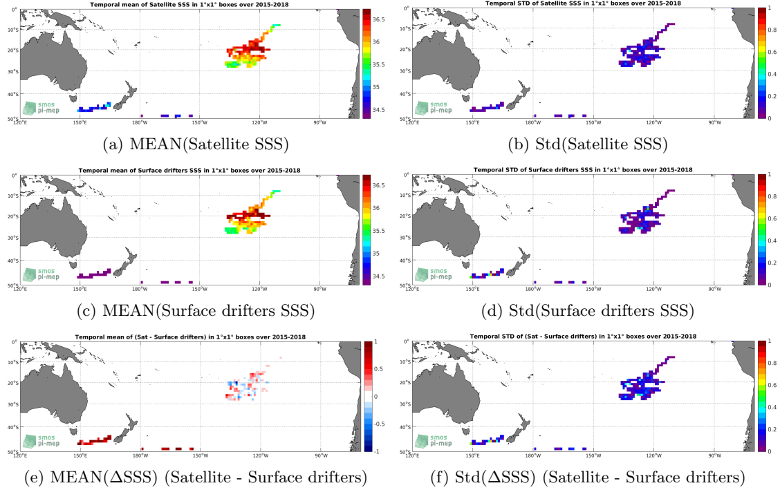
Figure 5: Temporal mean (left) and Std (right) of SSS from SMAP-L3-RSS-V4-8DAY-RUNNING (top), Surface drifters (middle), and of \Delta SSS (Satellite - Surface drifters). Only match-up pairs are used to generate these maps.
