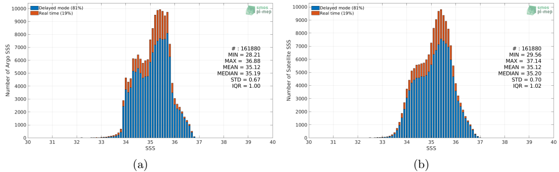
Figure 2: Histograms of SSS from Argo (a) and SMAP SSS L3 v4 - 8-Day running (RSS) (b) considering all match-up pairs per bins of 0.1 over the South Pacific Ocean Pi-MEP region and for the full satellite product period.
