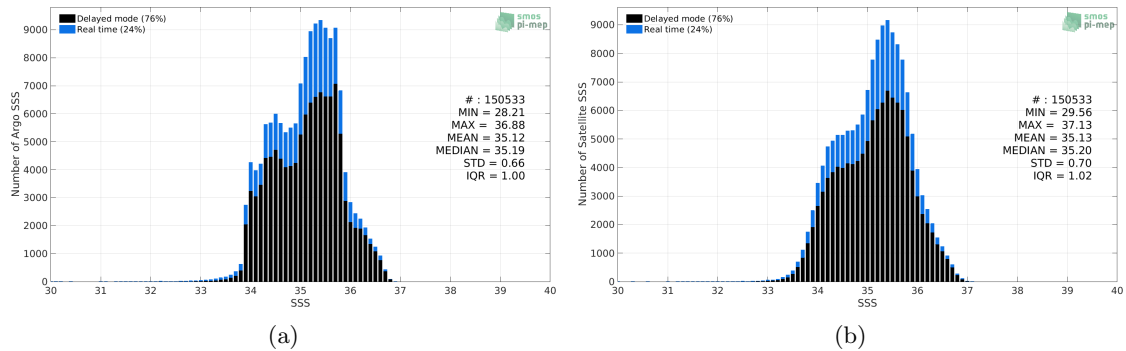
Figure 2: Histograms of SSS from Argo (a) and SMAP SSS L3 v4 - 8-Day running (RSS) (b) considering all match-up pairs per bins of 0.1 over the South Pacific Ocean Pi-MEP region and for the full satellite product period.
