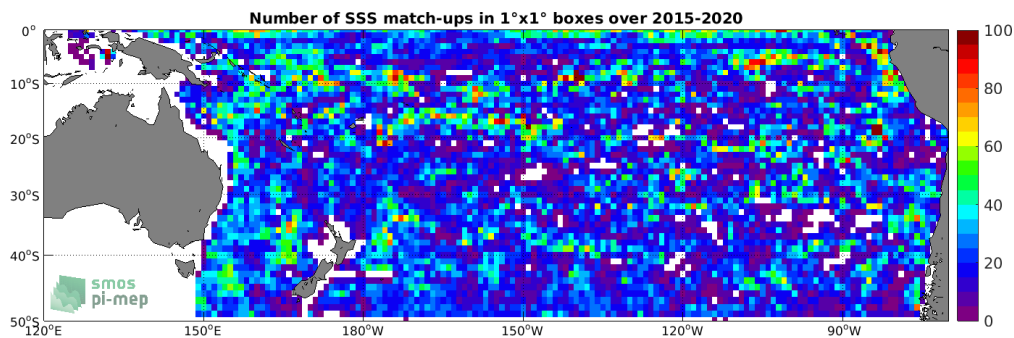
Figure 4: Number of SSS match-ups between Argo SSS and the SMAP SSS L3 v4 - 8-Day running (RSS) SSS product for the South Pacific Ocean Pi-MEP region over 1^\circ \times 1^\circ boxes and for the full satellite product period.
