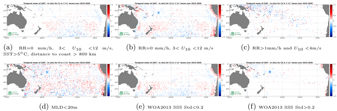
Figure 12: Temporal mean gridded over spatial boxes of size 1^\circ \times 1^\circ of \Delta SSS (SMAP SSS L3 v4 - 8-Day running (RSS) - Argo) for 6 different subdatasets corresponding to:RR=0 mm/h, 3 < U_{10} < 12 m/s, SST >5^\circ\text{C} , distance to coast > 800 km (a), RR=0 mm/h, 3 < U_{10} < 12 m/s (b), RR >1 mm/h and U_{10} < 4 m/s (c),MLD <20 m (d),WOA2013 SSS Std <0.2 (e),WOA2013 SSS Std >0.2 (f).
