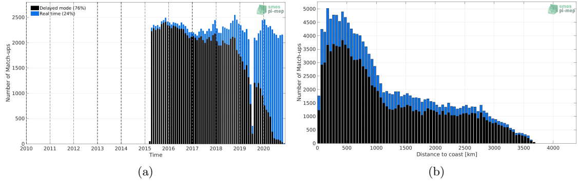
Figure 1: Number of match-ups between Argo and SMAP SSS L3 v4 - 8-Day running (RSS) SSS as a function of time (a) and as function of the distance to coast (b) over the South Pacific Ocean Pi-MEP region and for the full satellite product period.
