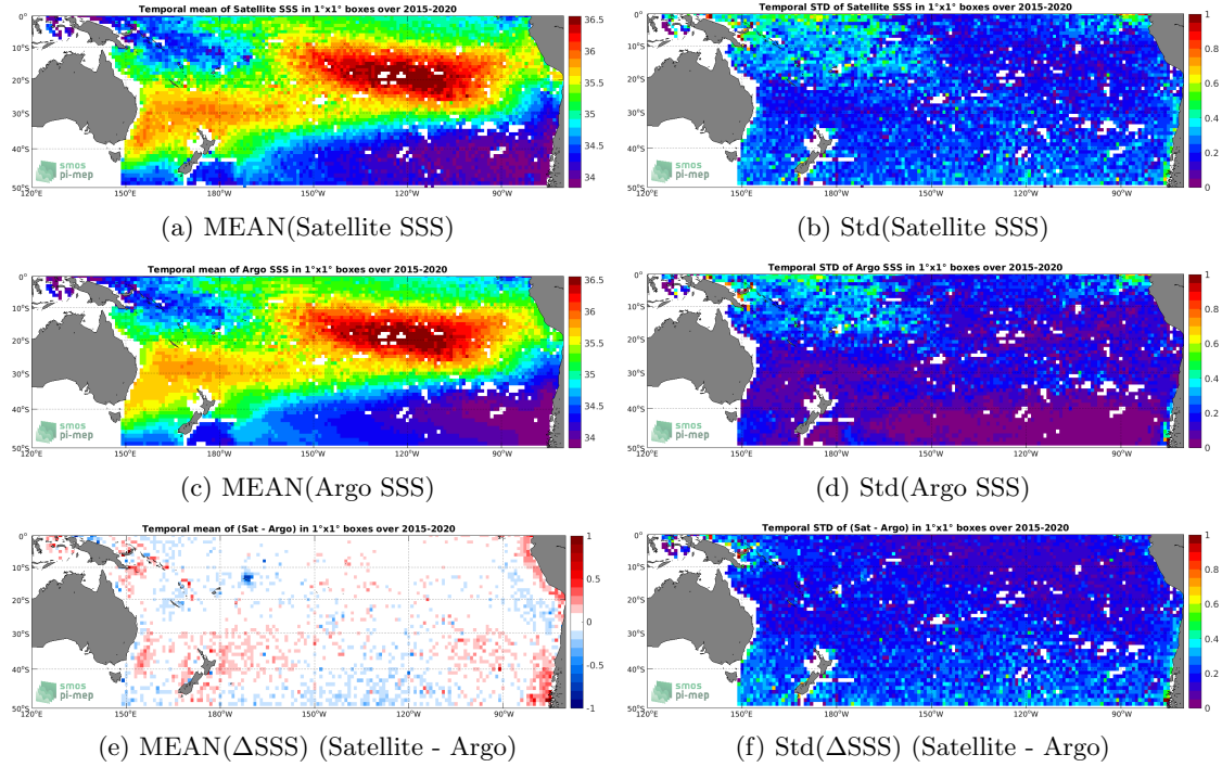
Figure 6: Temporal mean (left) and Std (right) of SSS from SMAP SSS L3 v4 - 8-Day running (RSS) (top), Argo (middle), and of \Delta SSS (Satellite - Argo). Only match-up pairs are used to generate these maps.
