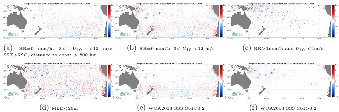
Figure 12: Temporal mean gridded over spatial boxes of size 1^\circ \times 1^\circ of \Delta SSS (SMAP-L3-RSS-V4-8DAY-RUNNING - Argo) for 6 different subdatasets corresponding to:RR=0 mm/h, 3 < U_{10} < 12 m/s, SST > 5^\circ\text{C} , distance to coast > 800 km (a), RR=0 mm/h, 3 < U_{10} < 12 m/s (b), RR > 1 mm/h and U_{10} < 4 m/s (c),MLD < 20 m (d),WOA2013 SSS Std < 0.2 (e),WOA2013 SSS Std > 0.2 (f).
