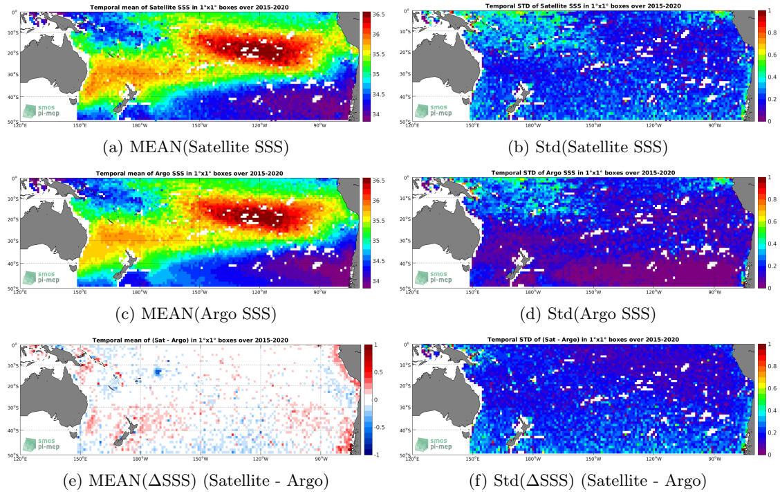
Figure 6: Temporal mean (left) and Std (right) of SSS from SMAP-L3-RSS-V4-8DAY-RUNNING (top), Argo (middle), and of \Delta SSS (Satellite - Argo). Only match-up pairs are used to generate these maps.
