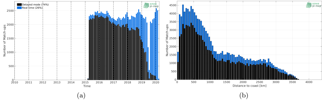
Figure 1: Number of match-ups between Argo and SMAP-L3-RSS-V4-8DAY-RUNNING SSS as a function of time (a) and as function of the distance to coast (b) over the South Pacific Ocean Pi-MEP region and for the full satellite product period.
