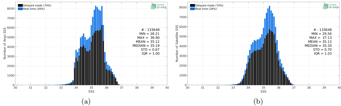
Figure 2: Histograms of SSS from Argo (a) and SMAP-L3-RSS-V4-8DAY-RUNNING (b) considering all match-up pairs per bins of 0.1 over the South Pacific Ocean Pi-MEP region and for the full satellite product period.
