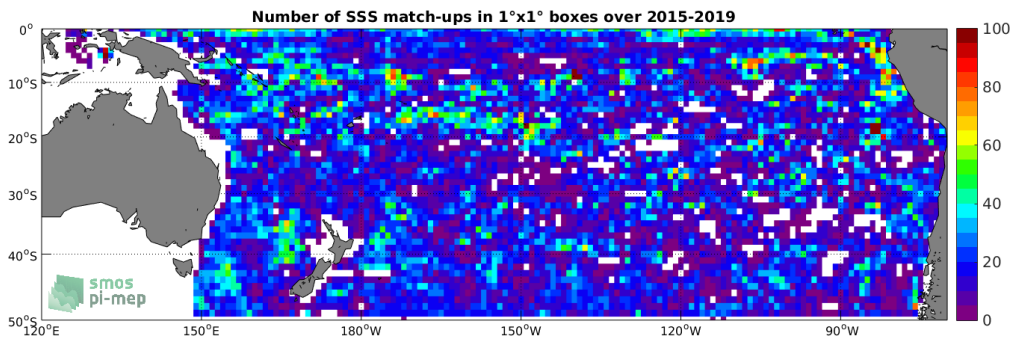
Figure 4: Number of SSS match-ups between Argo SSS and the SMAP-L3-RSS-V4-8DAY-RUNNING SSS product for the South Pacific Ocean Pi-MEP region over 1^\circ \times 1^\circ boxes and for the full satellite product period.
