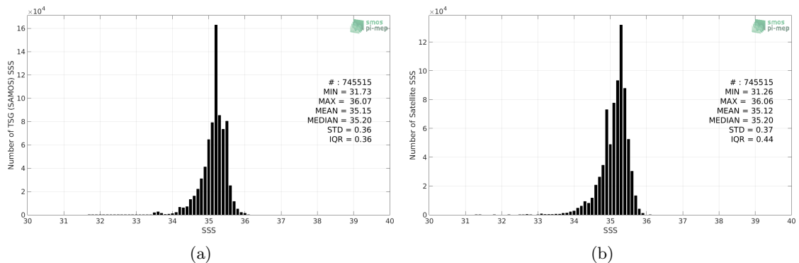
Figure 2: Histograms of SSS from TSG (SAMOS) (a) and SMAP SSS L3 v4 - Monthly (RSS) (b) considering all match-up pairs per bins of 0.1 over the South Pacific Ocean Pi-MEP region and for the full satellite product period.
