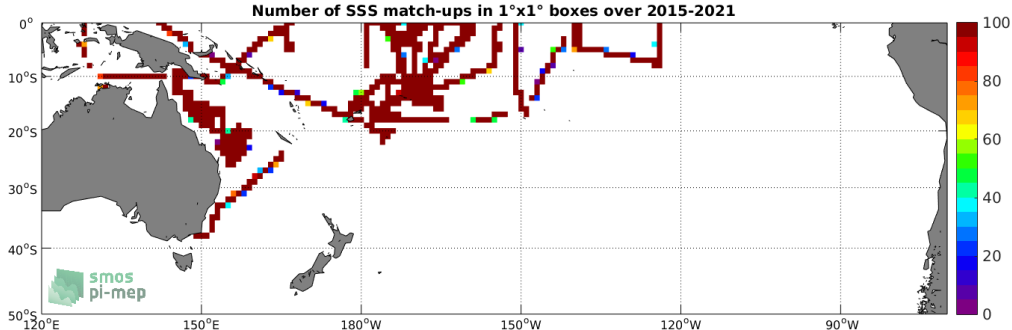
Figure 4: Number of SSS match-ups between TSG (SAMOS) SSS and the SMAP SSS L3 v4 - Monthly (RSS) SSS product for the South Pacific Ocean Pi-MEP region over 1^\circ \times 1^\circ boxes and for the full satellite product period.
