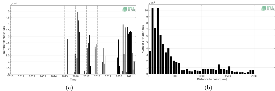
Figure 1: Number of match-ups between TSG (SAMOS) and SMAP SSS L3 v4 - Monthly (RSS) SSS as a function of time (a) and as function of the distance to coast (b) over the South Pacific Ocean Pi-MEP region and for the full satellite product period.
