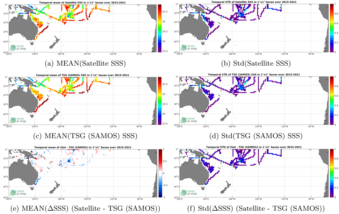
Figure 6: Temporal mean (left) and Std (right) of SSS from SMAP SSS L3 v4 - Monthly (RSS) (top), TSG (SAMOS) (middle), and of \Delta SSS (Satellite - TSG (SAMOS)). Only match-up pairs are used to generate these maps.
