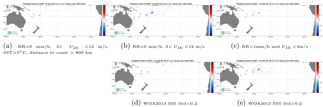
Figure 12: Temporal mean gridded over spatial boxes of size 1^\circ \times 1^\circ of \Delta\text{SSS} (SMAP SSS L3 v4 - Monthly (RSS) - TSG (SAMOS)) for 5 different subdatasets corresponding to:RR=0 mm/h, 3 < U_{10} < 12 m/s, SST >5^\circ\text{C} , distance to coast > 800 km (a), RR=0 mm/h, 3 < U_{10} < 12 m/s (b), RR >1 mm/h and U_{10} < 4 m/s (c), WOA2013 SSS Std <0.2 (d), WOA2013 SSS Std >0.2 (e).
