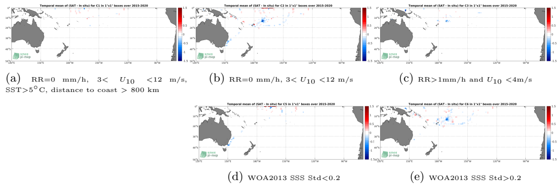
Figure 12: Temporal mean gridded over spatial boxes of size 1^\circ \times 1^\circ of \Delta SSS (SMAP-L3-RSS-V4-MONTHLY - TSG-SAMOS) for 5 different subdatasets corresponding to:RR=0 mm/h, 3 < U_{10} < 12 m/s, SST >5^\circ C, distance to coast > 800 km (a), RR=0 mm/h, 3 < U_{10} < 12 m/s (b), RR >1 mm/h and U_{10} < 4 m/s (c), WOA2013 SSS Std <0.2 (d), WOA2013 SSS Std >0.2 (e).
