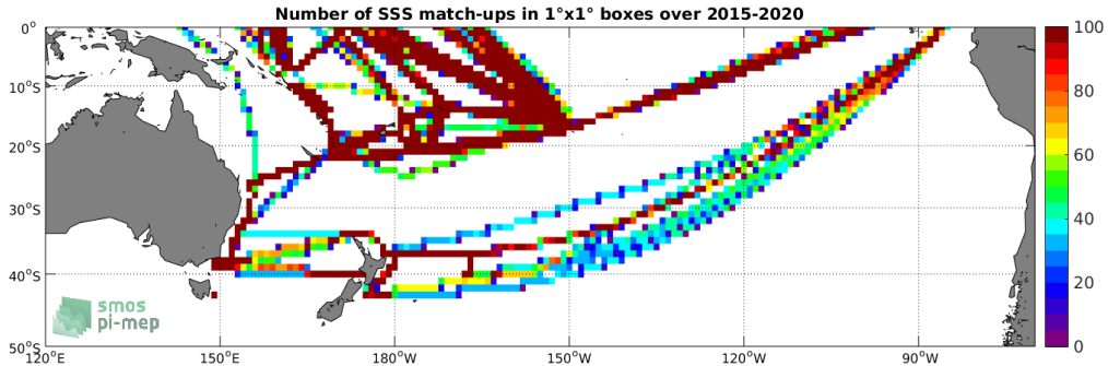
Figure 4: Number of SSS match-ups between TSG (LEGOS-DM) SSS and the SMAP SSS L3 v4 - Monthly (RSS) SSS product for the South Pacific Ocean Pi-MEP region over 1^\circ \times 1^\circ boxes and for the full satellite product period.
